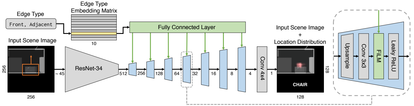
Fig. 9. Architecture of our graph-conditional location prediction network. We use a fully-convolution network (FCN) architecture to predict a 2D distribution of possible object locations, in the relative coordinate frame of an anchor object (orange region in the input image). The network’s output is conditioned on a type of relationship edge via featurewise linear modulation (FiLM) [Perez et al. 2018]. The network simultaneously predicts distributions for all categories; here we visualize the slice for “chair.”
