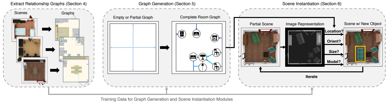
Fig. 2. Our scene synthesis pipeline. We automatically extract relation graphs from scenes (Section 4), which we use to train a deep generative model of such graphs (Section 5). In this figure, the graph nodes are labeled with an icon indicating their object category. We then use image-based reasoning to instantiate a graph into a concrete scene by iterative insertion of 3D models for each node (Section 6).
