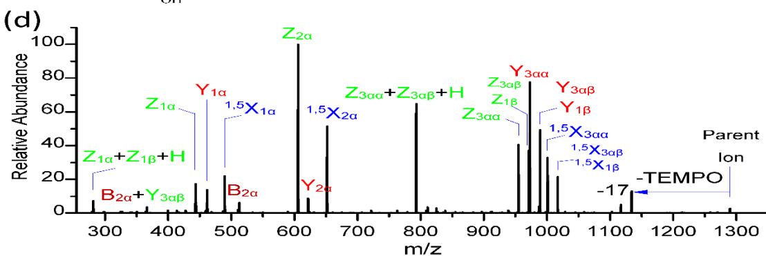
Figure 3. The fragmentation patterns observed following MS 2 CID of MNPs-FRAGS-derivatized LNDFH I (a), LNDFH II (c), and the CID spectra of MNPs-FRP-derivatized LNDFH I (b), LNDFH II (d).
