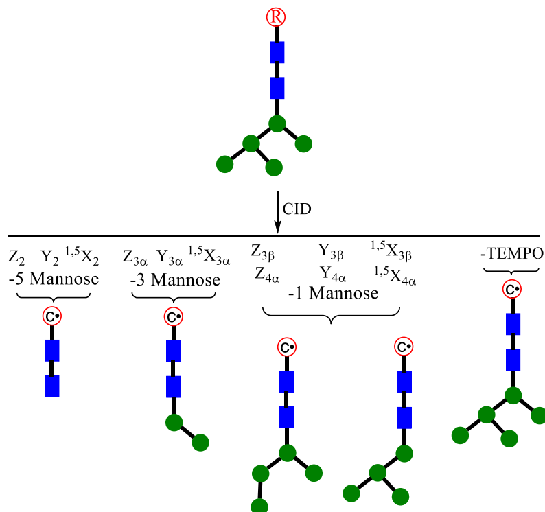
Figure 7. Radical-driven glycan deconstruction (R-DECON) diagram for \text{Man}_5\text{GlcNAc}_2 .
