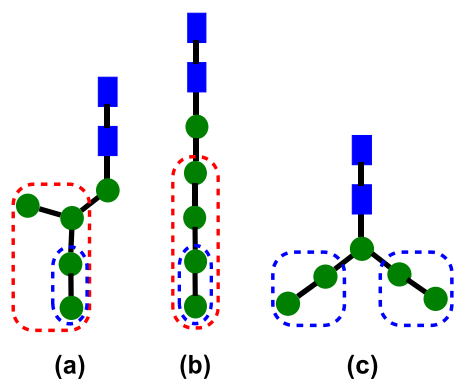
Figure 8. Proposed structures of \text{Man}_5\text{GlcNAc}_2 that would be able to lose two (enclosed in blue box) or four (enclosed in red box) mannose residues. Structures (a), containing one branch with one and three mannose residues on two sides, can have loss of two and four mannose residues. Structure (b) with no branches can have loss of two and four mannose residues. Structure (c), containing one branch with two mannose residues on each side, can have loss of two mannose residues.
