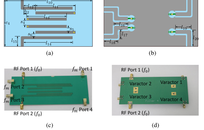
Fig. 10. Geometry of the fourth order filter designed in microstrip technology. (a) Detail of the top metalization layer. (b) Detail of the bottom metalization layer. Panels (c)-(d) show a picture of the top and bottom metalization layers of the fabricated prototype, respectively.
