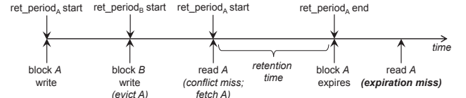
Figure 3: Illustration of expiration misses. Assume that blocks A and B are in the same memory location, i.e., a write from one block would evict the currently resident block
