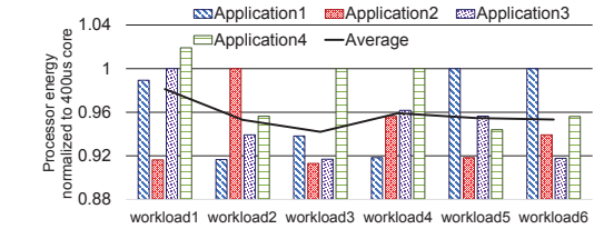
Figure 13: ARC energy savings in a multi-programmed scenario. We present results assuming no performance constraints are specified. If the predicted core is occupied, the next best available core is selected
