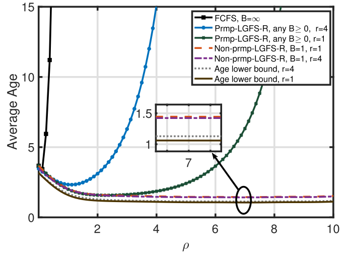
Fig. 6. Average age versus traffic intensity \rho for an update system with m = 4 servers, queue size B , maximum replication degree r , and i.i.d. NBU service times.
