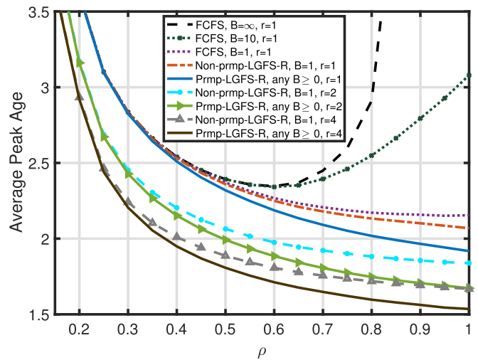
Fig. 4. Average peak age versus traffic intensity \rho for an update system with m = 4 servers, queue size B , maximum replication degree r , and i.i.d. exponential service times.
