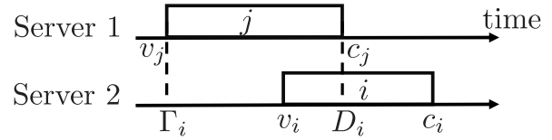
Fig. 8. An illustration of v_i , c_i , \Gamma_i , and D_i . There are 2 servers, and s_j > s_i . There is no packet with generation time greater than s_i that is assigned to any of the servers before time v_j . Packet j is assigned to Server 1 at time v_j and delivered to the destination at time c_j ; while packet i is assigned to Server 2 at time v_i and delivered to the destination at time c_i . The service starting time and completion time of packet j are earlier than those of packet i . Thus, we have \Gamma_i = v_j and D_i = c_j .
