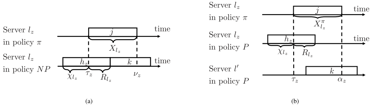
Fig. 10. The possible cases to occur after the completion of packet h_z . (a) Case 1: Packet k is assigned to server l_z after the completion of packet h_z . (b) Case 2: Packet k is assigned to server l' before the completion of packet h_z .
