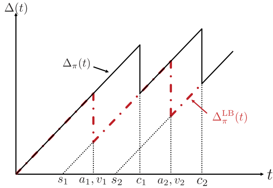
Fig. 5. The evolution of \Delta_\pi^{\text{LB}} and \Delta_\pi in a single server queue. We assume that a_1 > s_1 and a_2 > c_1 > s_2 . Thus, we have v_1 = a_1 and v_2 = a_2 .
