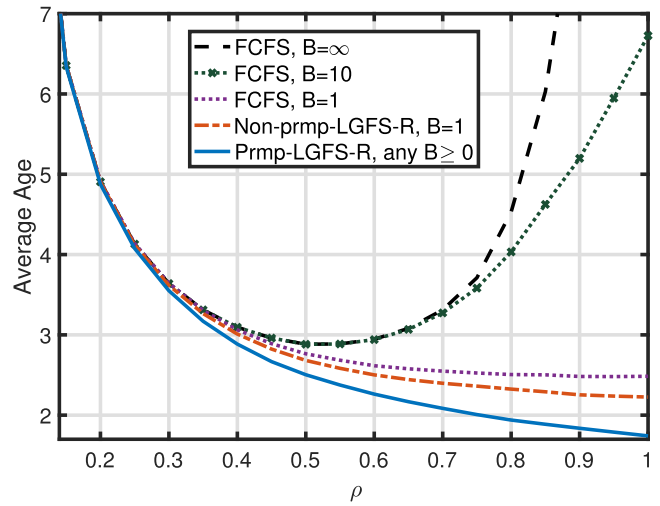
Fig. 3. Average age versus traffic intensity \rho for an update system with m = 1 server, queue size B , and i.i.d. exponential service times.
