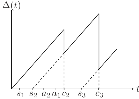
Fig. 2. Sample path of the age process \Delta(t) .
