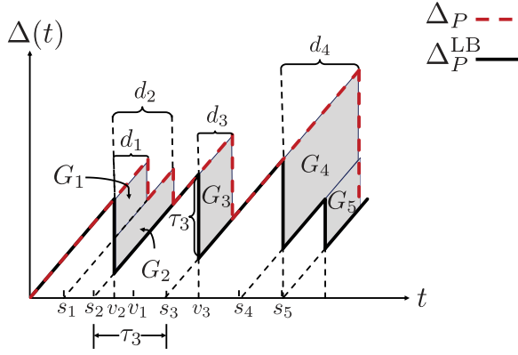
Fig. 11. The evolution of \Delta_P^{\text{LB}} and \Delta_P in a queue with 4 servers and r = 2 .
