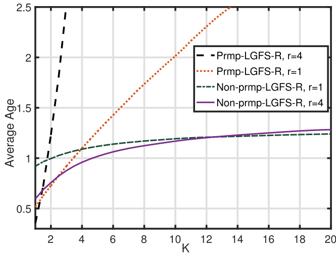
Fig. 7. Average age under gamma service time distributions with different shape parameter K , where m = 4 servers, queue size B = \infty , and maximum replication degree r .
