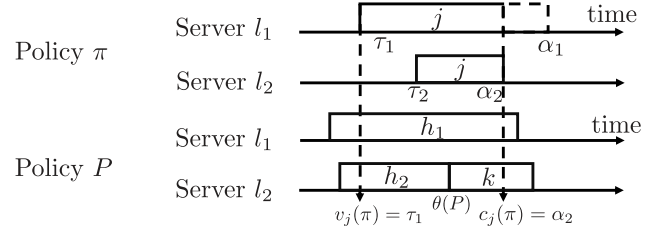
Fig. 9. Illustration of packet assignments under policy \pi and policy P . In policy \pi , two copies of packet j are replicated on the server l_1 and server l_2 at time \tau_1 and \tau_2 , where v_j(\pi) = \min\{\tau_1, \tau_2\} = \tau_1 . Server l_2 completes one copy of packet j at time c_j(\pi) = \alpha_2 , server l_1 cancels its redundant copy of packet j at time c_j(\pi) . Hence, the service duration of packet j is [v_j(\pi), c_j(\pi)] in policy \pi . In policy P , at least one of the servers l_1 and l_2 becomes idle before time c_j(\pi) . In this example, server l_2 becomes idle at time \theta(P) < c_j(\pi) and a fresh packet k with s_k \geq s_j starts its service on server l_2 at time \theta(P) .
