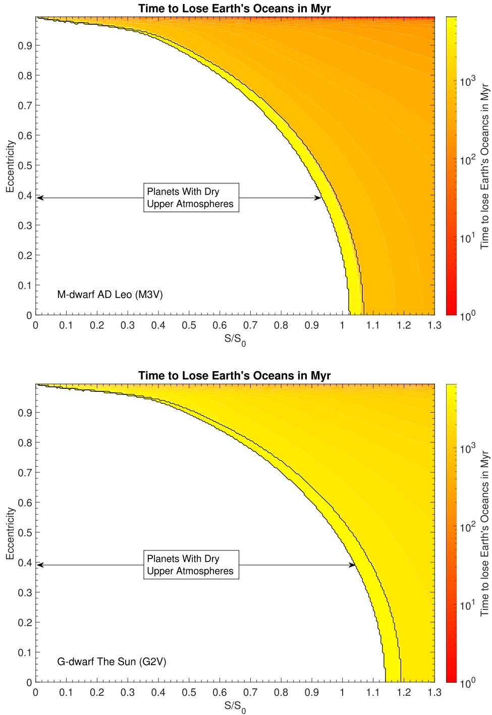
Figure 6. Time to lose Earth’s entire surface water inventory on aqua planets orbiting M-dwarf AD Leo and G-dwarf star the Sun in Myr. The M-dwarf planet is exposed to \sim 6\times more XUV flux than the G-dwarf planet with an equivalent climate, leading to a \sim 6\times higher mass loss rate. The black contour outlines the boundaries of the moist GH.
