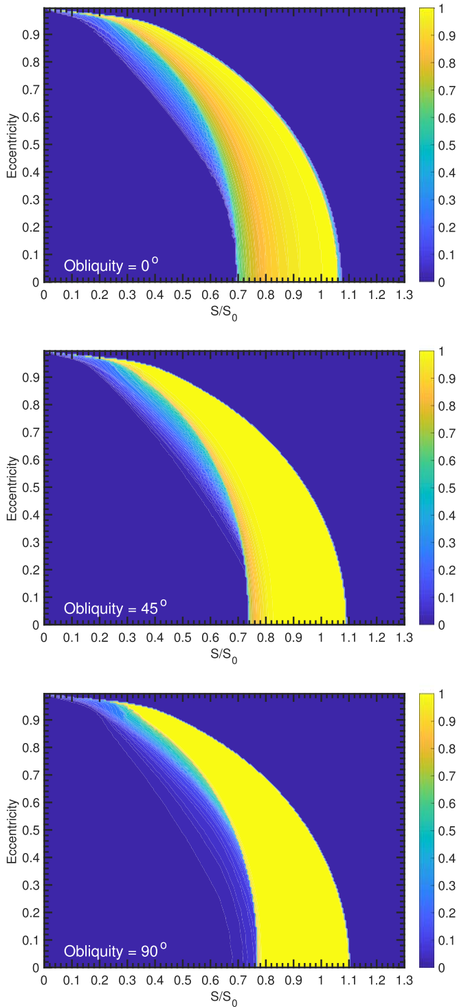
Figure 9. Fractional habitability on an M-dwarf planet with 0°, 45°, 90° obliquity, after EBM simulations assuming warm-start conditions.
