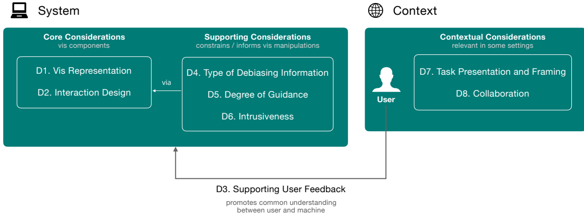
Figure 1: The design space is comprised of 8 dimensions, described in Section 3. D1 (VISUAL REPRESENTATION) and D2 (INTERACTION DESIGN) are the two core components of a visualization [13] that can be manipulated to mitigate biased decision making processes. How these components are manipulated is informed and constrained by supporting considerations, including D4 (TYPE OF DEBIASING INFORMATION), D5 (DEGREE OF GUIDANCE) and D6 (INTRUSIVENESS). Some contextual considerations may only be relevant in specific settings, including D7 (TASK PRESENTATION AND FRAMING) and D8 (COLLABORATION). Finally, D3 (SUPPORTING USER FEEDBACK) connects the user and contextual setting to the system by promoting a common understanding between user and machine.
