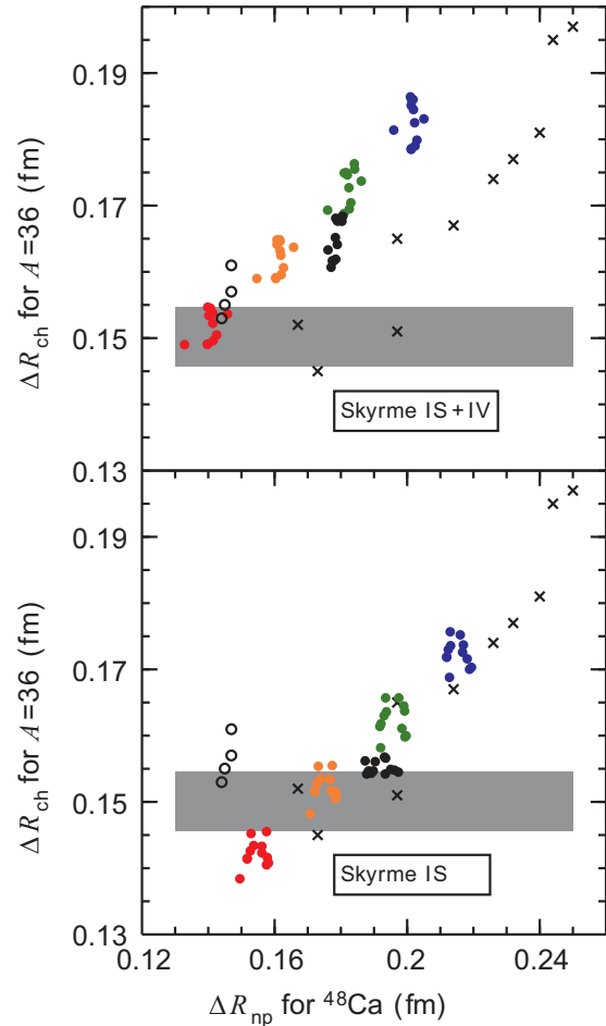
FIG. 3. The correlation between \Delta R_{\text{ch}} for A = 36 and the neutron skin of ^{48}\text{Ca} . The symbols are the same as in Figs. 1 and 2.
