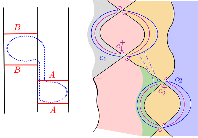
FIGURE 4. Left: Pattern in the state graph exhibiting a non-trivial Stallings twist. Right: The curve c obtained as a connected sum of the curves c_1, c_2 with self linking +2 and -2 .
