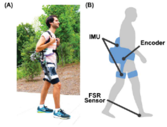
Fig. 1. Powered bilateral hip exoskeleton. (A) The device can provide power assistance along the sagittal plane. The user interface can be adjusted to accommodate different user body sizes. (B) Multiple mechanical sensors are placed on the device to measure the user's movement. The IMUs are placed one on the trunk and one on each thigh segment, encoders are located at the hip joint bilaterally, and the FSR sensors are placed at each heel of the user.
