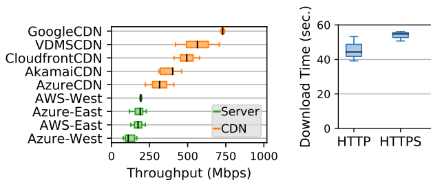
Figure 16: HTTP(S) download throughput for 9 CDN/cloud servers over 5G. Figure 17: 5G download time (1 GiB file) over HTTP vs. HTTPS.
