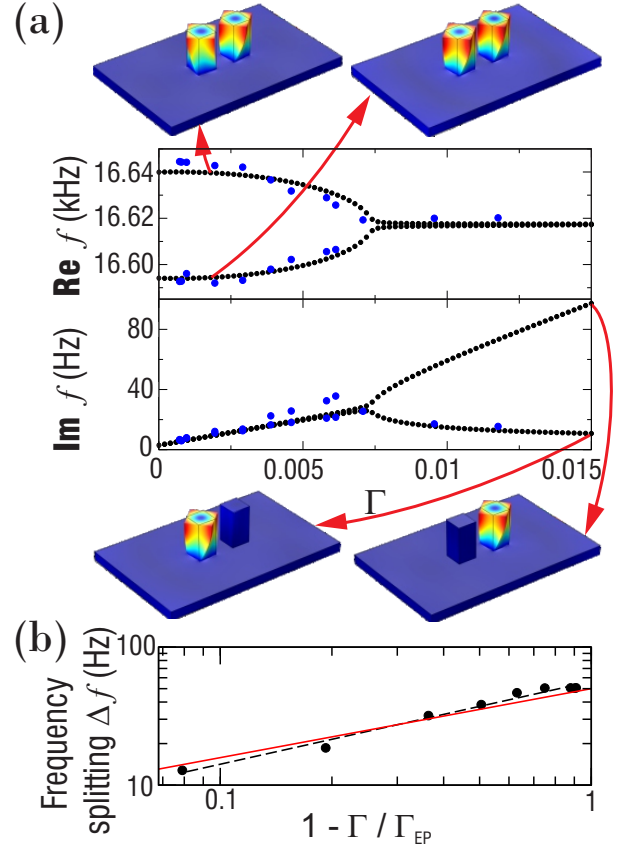
FIG. 4. (a) Numerical calculations (black dots) and experimental data (blue dots) of the real and imaginary parts of the eigenfrequencies of the two pillars oscillating in their first torsional modes as a function of the loss parameter \Gamma . The experimental results are in a good agreement with the numerical simulation. In the same sub-figure we report the modes of the system for two typical cases of the differential loss \Gamma . (b) Log-log plot of the measured frequency splitting \Delta f versus 1 - \Gamma/\Gamma_{EP} near the exceptional point. The red solid line shows the square-root law \delta f \sim \sqrt{1 - \Gamma/\Gamma_{EP}} while the black dashed line is the best linear fit (1 - \Gamma/\Gamma_{EP})^\alpha with \alpha \approx 0.6 .
