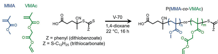
Scheme 1 RAFT copolymerization of methyl methacrylate (MMA) and vinyl methacryloxy acetate (VMAc).
