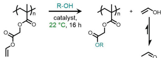
Fig. 1 (A) Previous work demonstrating efficient transesterification of poly(methyl acrylate) via removal of methanol at elevated temperature. (B) Proposed method leveraging keto–enol tautomerization to promote side-chain functionalization.
