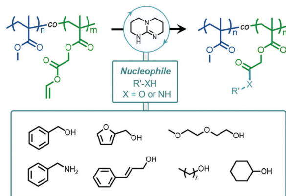
Scheme 2 General scheme for TBD-catalyzed transesterification and amidation of P(MMA-co-VMAc) in the presence of various functional nucleophiles.
