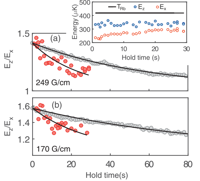
FIG. 2. Cross-dimensional relaxation of ^7\text{Li} atoms within a co-trapped ^{87}\text{Rb} gas. Red circles show the measured kinetic energy ratio ( E_z/E_x ) for the lithium gas. Gray circles show results of Monte Carlo simulations accounting for experimental parameters and the theoretically predicted energy-dependent differential cross section derived using the ^7\text{Li} - ^{87}\text{Rb} molecular potential modeled in Ref. [5]. Results at two trap strengths are shown: B' = 249 G/cm (a) and B' = 170 G/cm (b). Inset: neither E_z (solid blue) nor E_x (hollow orange), at B' = 249 G/cm trap strength, reaches the isotropic kinetic energy of the cotrapped rubidium gas (solid black line) during the accessible evolution time.
