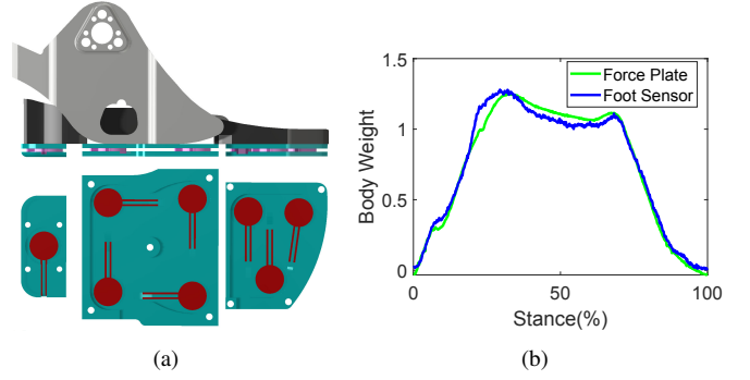
Fig. 2. (a) Sagittal view of Comex foot plate (top) shows the rigid structure (gray), insole (black), force sensor plates (green), and force-channeling pucks (purple). Top-down view (bottom) shows the layout of FSRs (red) within the sensor plates (green). (b) Comparison of simultaneously recorded foot sensor and force plate readings for one stance period during level-ground walking. Both signals are normalized to body weight and temporally normalized to percent stance period. A correlation coefficient of 0.99 and a mean squared error of 0.03 were found between the two signals.
