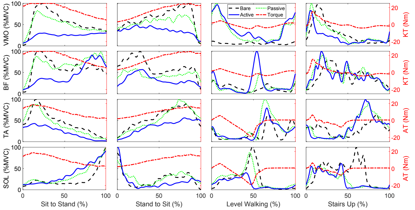
Fig. 4. Comparisons of mean EMG between the three exoskeleton modes tested (bare, passive, and active), along with the assistance torque for the corresponding joint. The four activities tested (sit to stand, stand to sit, level walking, and stairs up) are shown column wise, whereas the four muscles tested (VMO, BF, TA, and SOL) are shown row wise. Rows one and two represent the muscles primarily responsible for controlling the knee joint and torque provided by Comex at the knee (KT). Rows three and four represent the muscles primarily responsible for controlling the ankle joint and the torque provided by Comex at the ankle (AT). A positive KT represents a knee extension torque, whereas a positive AT represents a dorsi-flexion torque.
