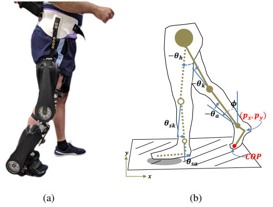
Fig. 1. (a) Comex exoskeleton worn by a healthy user. (b) Kinematic model of the body reproduced from [22]. COP denotes the center of pressure, solid links denote the stance leg, and dashed links denote the swing leg.
