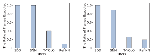
(a) Car detection ( TOR=0.435 ) (b) Person detection ( TOR=0.259 )
