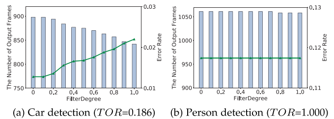
Fig. 10. The throughput and error rate as a function of FilterDegree .
