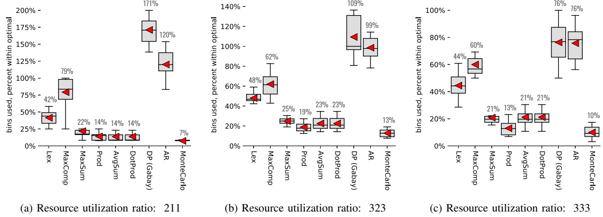
Fig. 2: Performance within optimal for case 1: low resource utilization variance, n = m = 100
