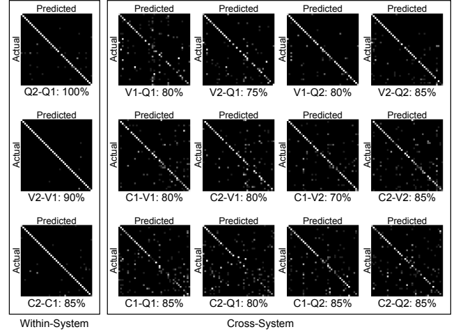
Figure 2: Confusion matrices for within-system and cross-system authentication for the highest accuracies per trajectory percentage.
