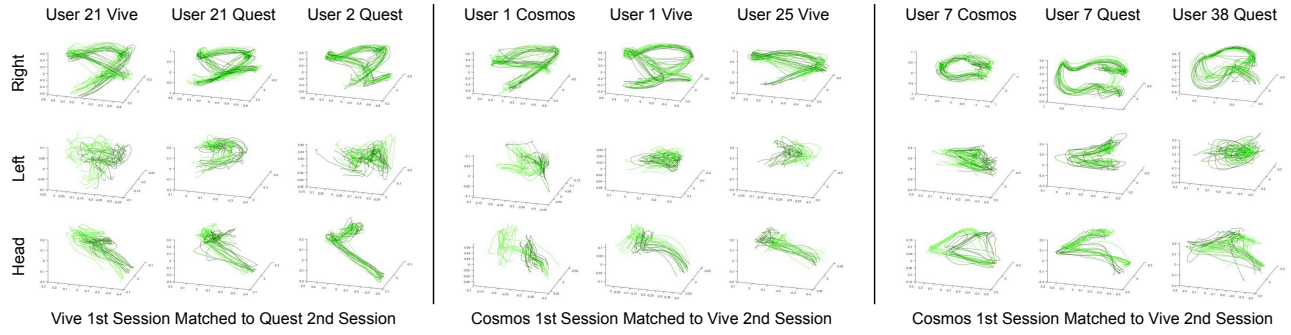
Figure 3: Users that misclassify (dark green trajectories of left columns of each panel) for a given VR system, and test user (light green trajectories of center columns) and confounding user (light green trajectories of right columns) for training VR system.
