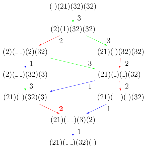
Figure 4: Partial filling of the connected component of \mathcal{H}^4(3) containing highest weight element ( ) (21) (32) (32) .
