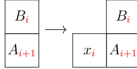
Figure 1: A forbidden case while inverting the residue map.
