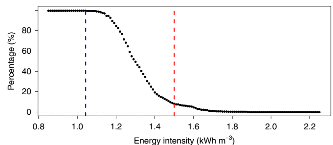
Fig. 4 | Percentage of distributed DPR system configurations that keep energy consumption lower than Baseline as a function of WWTP energy intensity. Red dashed line indicates mid-case energy intensity of 1.5 \text{ kWh m}^{-3} considered in this study. Blue dashed line indicates the energy intensity below which 100% of the configurations achieve net energy saving.
