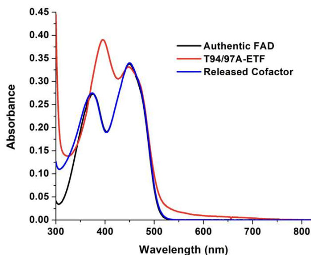
Figure 2: Visible spectra of T94/97A ETF and cofactors released from it, showing that the released flavin has a spectrum similar to authentic FAD whereas its signal when bound in purified 37.6 \mu\text{M} T94/97A ETF protein is perturbed, reflecting interactions with the protein environment.
