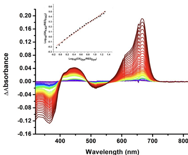
Figure 5: Difference spectra observed in the course of reductive titration of T94/97A ETF (374 and 450 nm) and methylene blue (664 nm). Each difference spectrum shown is an observed spectrum minus the spectrum at the end of the first phase of reduction (Figure 4). The difference spectra thus emphasize changes associated with the reduction of OX to ASQ. Inset: plot of \log([OX]_{dye}/[RED]_{dye}) vs. analogous quantity for the flavin of T94/97A ETF, illustrating linear behaviour consistent with the Nernst equation. The slope near 0.5 is consistent with a 1-e - event. The best fit is y=0.491x-0.126 . R^2 = 0.996 .
