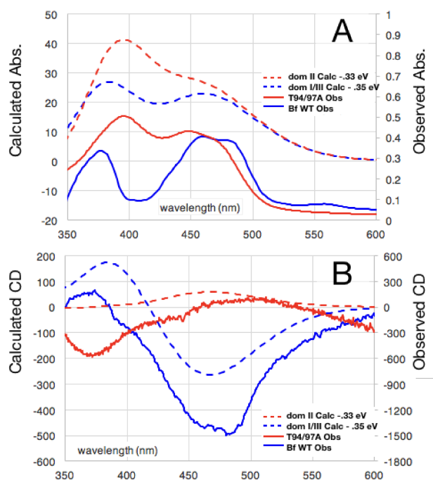
Figure 6: Comparison of observed vs. computed spectra. Absorbance data are in panel A whereas CD spectra are in B. Spectra of OX T94/97A ETF (red) are compared with those of the Bf-FAD (blue) collected on WT Rpa ETF in which contributions from the ET-FAD were suppressed by chemical reduction (i.e. only the Bf-FAD remains in the strongly absorbing OX state). Calculated spectra are based on a TD-DFT computations using B3LYP and the 6-31++G(d,p) basis with quantum treatment of the domII active site (55 atoms, Supplemental Figure S5) or the domI/III active site (50 atoms, Supplemental Figure S5). See supplemental Figure S6 for an example of the individual transitions contributing to these envelopes and the effects of different sizes of quantum zones.
