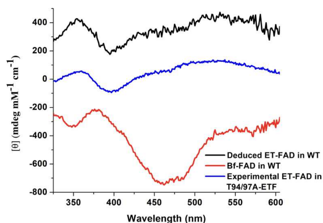
Figure 3: Visible CD spectrum of T94/97A ETF (in blue) in the oxidized (OX) state, compared with control spectra. These are (in red) the spectrum of WT RpaETF in which only the Bf-FAD is OX (the ET-FAD is HQ and therefore makes very little contribution), and (in black) the CD signal of the ET-FAD from WT RpaETF . The latter was obtained by collecting the CD spectrum of fully OX RpaETF and then subtracting away the contribution of Bf-FAD (red) to reveal the contribution of the ET-FAD. 3 The CD spectrum of the FAD in T94/97A ETF shows better agreement with the ET-FAD CD signal vs. the Bf-FAD CD signal. Note that vertical offsets of \pm 250 were applied to the two WT RpaETF signals in order to avoid overlap with the spectrum of T94/97A ETF.
