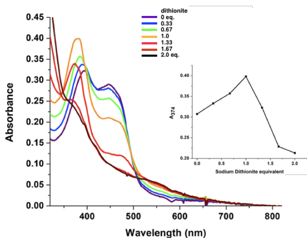
Figure 4: Visible spectra observed in the course of stepwise reduction of T94/97A ETF with dithionite, and plot of the absorbance ( A_{374} ) illustrating the change in the nature of the reaction after dithionite exceeded 1 equiv. In the first phase of reduction A_{374} increases, whereas in the second it decreases. The concentration of ETF-bound FAD was 34 \mu M.
