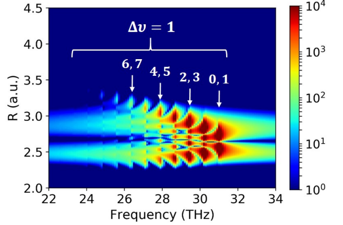
FIG. 5. Vibrational quantum-beat spectrum for the field-free evolution of the nuclear probability density in the binding \text{O}_2^+(a^4\Pi_u) BO state. Selected pairs of beating vibrational states are indicated by short white arrows and corresponding vibrational quantum numbers.
