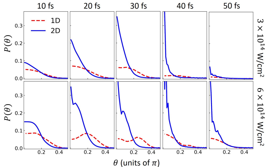
FIG. 2. Angular distribution of \text{O}^+ fragments for 50 fs delayed 800 nm probe laser pulses with peak intensities of 3 \times 10^{14} \text{ W/cm}^2 (upper panels) and 6 \times 10^{14} \text{ W/cm}^2 (lower panels) and pulse durations between 10 fs and 50 fs (from left to right). Dashed red and solid blue curves are results for calculations without (1D) and including rotational excitation (2D), respectively.
