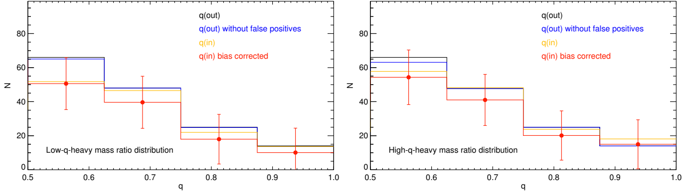
Figure 10. Raw and corrected mass ratio distributions for NGC 188 main sequence binaries, assuming a low- q -heavy (left) and high- q -heavy (right) mass ratio distribution. The raw output mass ratio distribution from the NGC 188 photometric catalog is shown in black in both panels. The results of all simulation runs together, shown in Fig. 6, are used to correct this distribution for false positives (blue), selection biases in output versus input mass ratio (orange), and finally, for detection incompleteness as a function of input mass ratio (red). Despite the assumption of two schematically different mass ratio distributions used to calculate the corrections, the q > 0.5 mass ratio distribution of NGC 188 consistently rises towards lower mass ratios.
