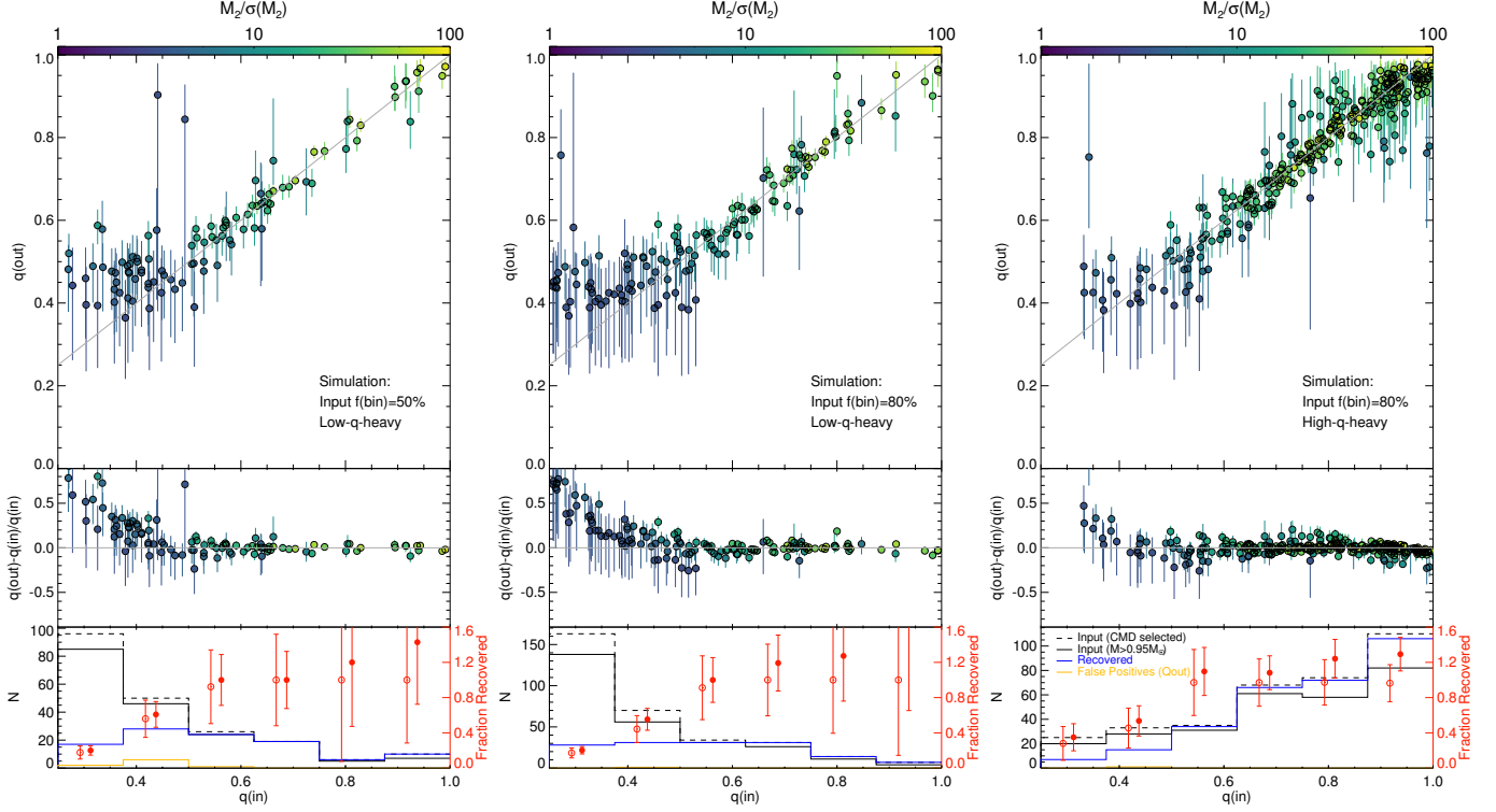
Figure 5. For main sequence binaries from the three example cases shown in Fig. 4, we plot recovered versus input mass ratio q (top) and its fractional residuals (middle), color coded by output M_2/\sigma(M_2) . In the bottom panel for each example case, we show histograms of the input mass ratio q(in) drawn from the primary-mass-limited sample ( M > 0.95M_\odot ) using solid black lines, while the input mass ratio distribution from the CMD-selected sample is shown using dotted black lines, illustrating that while the CMD-selected sample is larger, the distributions of q(in) are similar. The q(in) distribution for the subset of the CMD-selected sample which was successfully recovered is shown in blue, and a histogram of the output mass ratios of input single stars misidentified as binaries (i.e. false positives) is shown in orange, clustered near q(out) \sim 0.4 regardless of binary fraction or mass ratio distribution. The fraction of input binaries which was successfully recovered as a function of q(in) is overplotted in red with Poissonian error bars, using open circles to illustrate the recovery fraction versus the CMD-selected sample (offset by \Delta q(in) = -0.02 for clarity), and filled circles to directly compare the ratio of recovered binaries from the CMD-selected sample to the number of input binaries from the larger primary-mass-selected sample.
