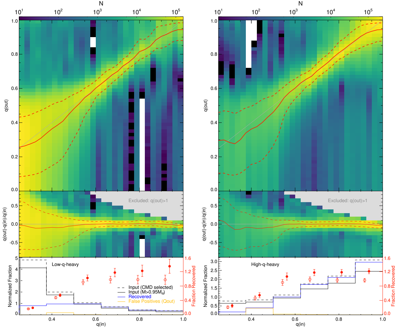
Figure 6. As in Fig. 5, but showing results from all MCMC iterations for all simulation runs concatenated together for the low- q -heavy (left) and high- q -heavy (right) mass ratio distributions. The red solid and dashed lines indicate the running median and 16th-84th fractiles respectively. The simulations indicate that both the accuracy and precision of recovered mass ratios suffer at low ( q < 0.5 ) mass ratios, while for q > 0.9 , input mass ratios are recovered to better than 10% at 1\sigma but are biased low due to output mass ratio distributions being truncated at an upper limit of q = 1 .
