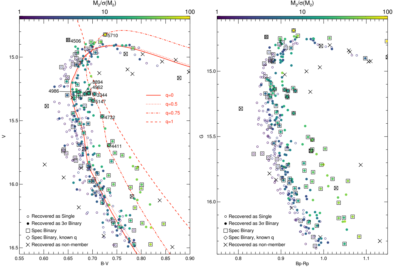
Figure 7. CMDs illustrating the results of a BASE-8 run on our observed photometric catalog of NGC 188 members, in the (B - V), V plane (left) and using Gaia DR2 photometry (right). Stars recovered as binaries, with M_2 > 3\sigma(M_2) (regardless of mass ratio) are shown as filled circles, and stars not recovered as binaries, with M_2 < 3\sigma(M_2) , are shown as small open circles. Stars are color coded by M_2/\sigma(M_2) as in Fig. 5. Known spectroscopic binaries from Geller & Mathieu (2012) are indicated by boxes, and those with spectroscopic mass ratios q(spec) are indicated with diamonds and labeled by their ID number in the left panel. Crosses indicate stars which were rejected as non-members by BASE-8. In the left panel, the best fit DSED isochrone is shown in red (solid line), and the resulting sequences corresponding to mass ratios of q=0.5, 0.75 and 1 are shown as red dotted, dot-dashed and dashed lines respectively.
