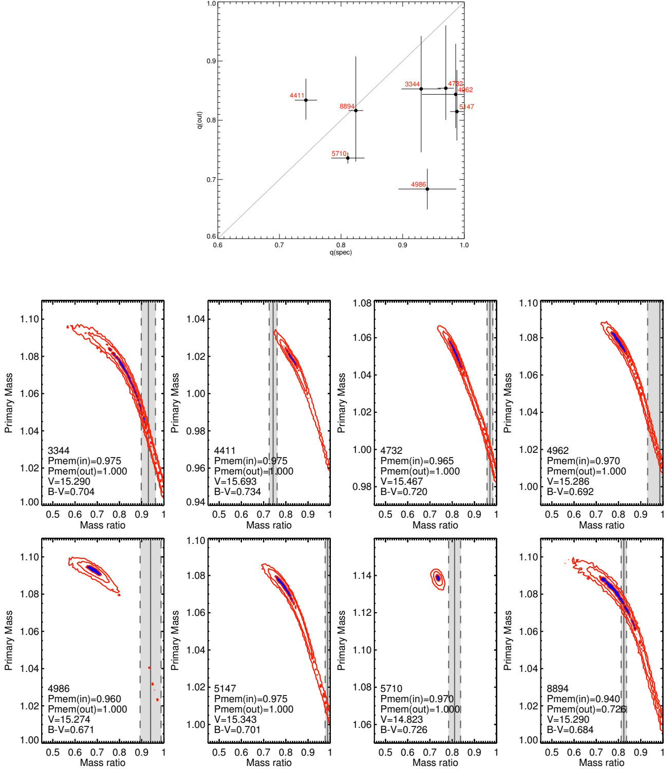
Figure 8. Top: For the 8 main sequence binaries with spectroscopic mass ratios from Geller & Mathieu (2012), a comparison of the mass ratios determined from our photometric catalog by BASE-8 versus the spectroscopic mass ratio. Points represent the median and error bars represent the 16th-84th fractile interval, and stars are labeled in red by their WOCS ID number corresponding to Fig. 7. Bottom: PDFs of primary mass versus mass ratio for each of the eight main sequence binaries with known spectroscopic mass ratios. The spectroscopic value and its uncertainty are indicated by the grey vertical solid and dashed lines respectively, and our recovered values are shown using contours of 3, 2 and 1 \sigma , with the latter shaded in blue. For each star, its ID number, its input (from proper motions and/or radial velocities) and output membership probability, and its (B - V) , V color and magnitude are given in the lower left. The y-axis values are shifted from star to star, but the scale of both axes is kept constant in all panels.
