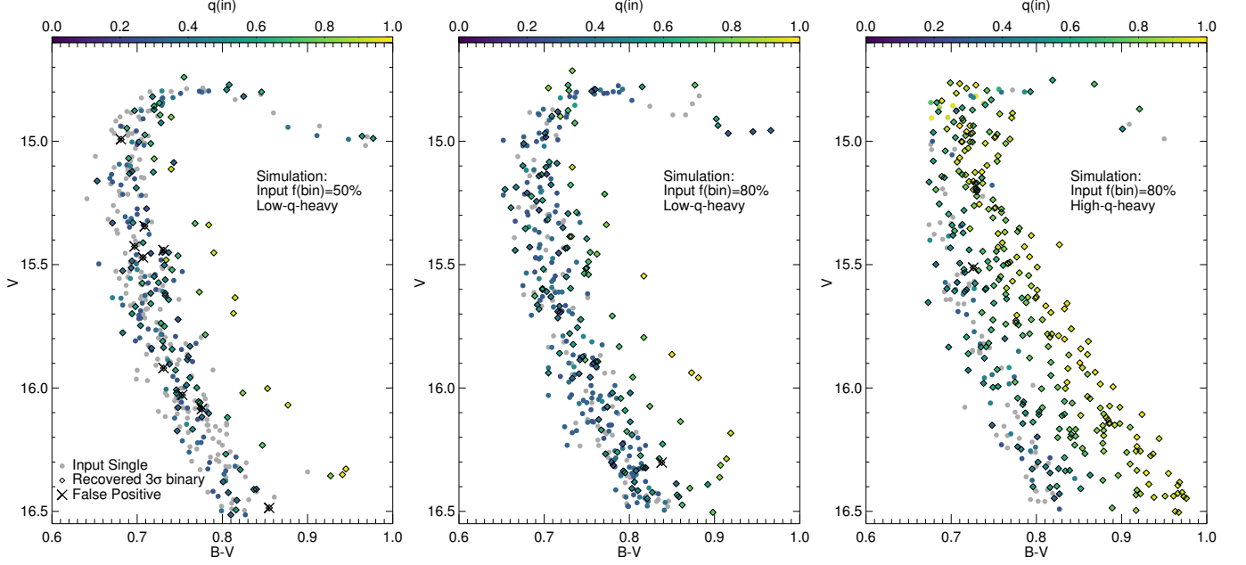
Figure 4. Example CMDs of simulated clusters in which stars are color-coded by their input mass ratio q(in) . Single stars are shown in grey, binaries successfully recovered by BASE-8 are marked with diamonds, and input singles misidentified as binaries are marked with crosses. The left and center panels compare two example cluster realizations, both with a low- q -heavy input mass ratio distribution but differing binary fractions of 50% (left) and 80% (center), while the center and right-hand panels compare two clusters with input binary fractions of 80% but different input mass ratio distributions.
