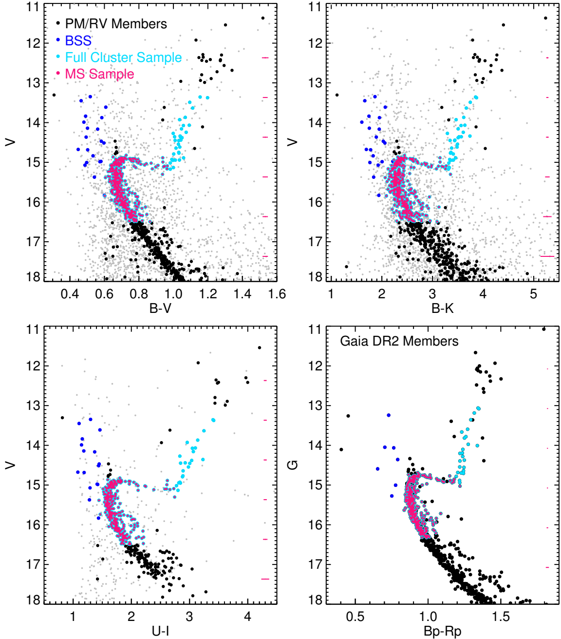
Figure 1. Color-magnitude diagrams in four color-magnitude planes, illustrating the full photometric catalog ( UBVRI from Stetson et al. 2004 and JHK_S from 2MASS). Stars in grey fail our 50% membership probability cut and are excluded from our analysis, and the remainder (black, blue, magenta and cyan) pass this cut. Blue circles are BSS from Gosnell et al. (2015) which are also excluded from our analysis. Cyan filled circles are included in our full cluster sample (used to derive cluster and stellar parameters), while only stars also in magenta are included in our analysis of the main sequence binary population. In the lower right panel, only members from Gaia Collaboration et al. (2018) are shown. Median photometric errors in magnitude bins are shown on the right-hand side of each CMD.
