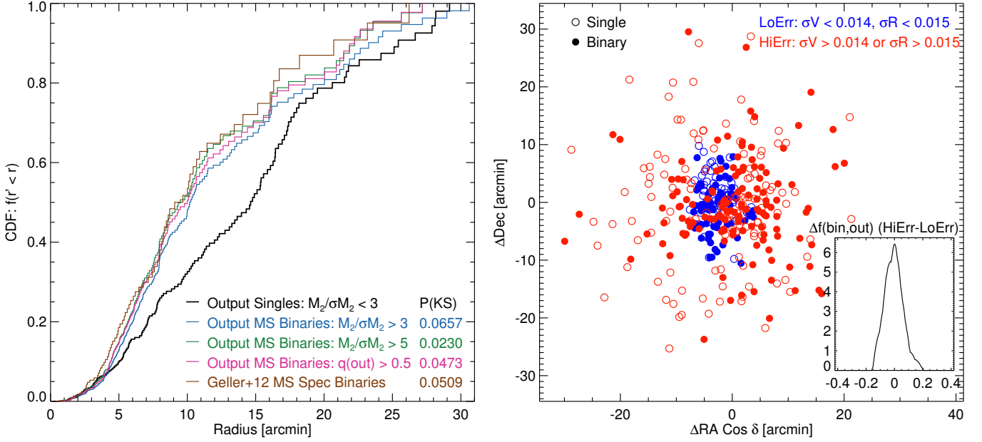
Figure 9. (Left:) Cumulative distribution functions comparing the radial positions of the single main sequence stars (thick black line) and binaries (blue line) in NGC 188. The binaries are identified as described in the main text, as those objects that have M_2 > 3\sigma(M_2) , and all other stars are considered single. More stringently selected binary samples, shown for comparison, have similar cumulative radial distributions to the M_2 > 3\sigma(M_2) sample. The results of a two-sided K-S test comparing the radial distributions of single stars to binaries is also given in the lower left corner for the various binary selection criteria, confirming that the ability of our method to recover the known mass segregation of binaries in NGC 188 is robust to the specifics of the binary selection criteria. (Right:) Positions of main sequence stars in NGC 188, color coded by photometric error, revealing that stars farther from the center of the cluster tend to have higher photometric errors. To test whether this could bias the radial distributions of recovered binaries shown in the left-hand panel, in the inset we show simulation results comparing the output binary fraction f(bin, out) over all runs for stars with higher versus lower photometric errors, as given in the upper right corner.
