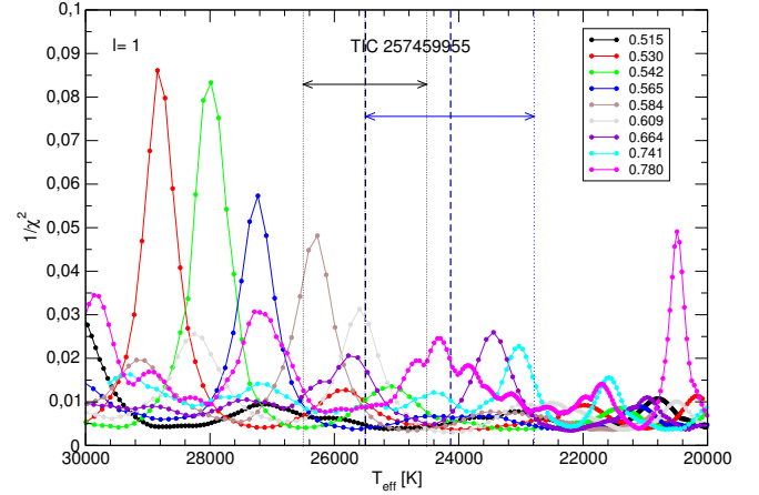
Fig. 7. Inverse of the quality function of the period fit in terms of the effective temperature for the case in which we assume that the modes are all \ell = 1 . The vertical black dashed line indicates the spectroscopic T_{\text{eff}} of TIC 257459955 and the vertical dotted lines its uncertainties according to Voss et al. (2007; T_{\text{eff}} = 25\,518 \pm 1000 K). Similarly, the blue vertical lines correspond to the spectroscopic T_{\text{eff}} and its uncertainties as derived by Rolland et al. (2018; T_{\text{eff}} = 24\,130 \pm 1369 K).
