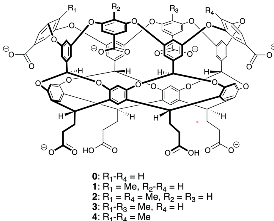
Fig. 1 Chemical structures of the hosts octa-acid ( 0 ), mono- endo -methyl octa-acid ( 1 ), 1,3-di- endo -methyl octa-acid ( 2 ), tri- endo -methyl octa-acid ( 3 ), tetra- endo -methyl octa-acid ( 4 ) used in this study.
