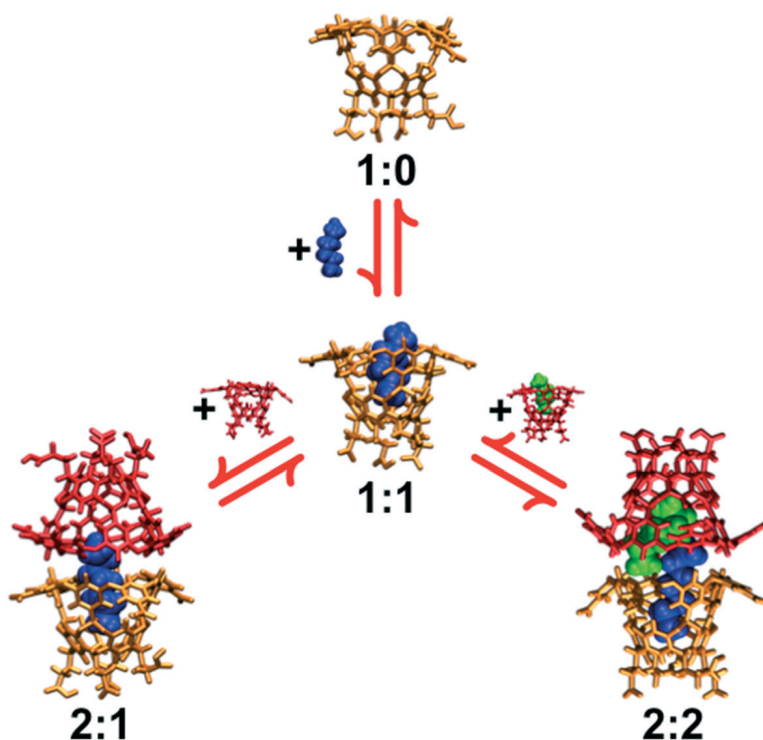
Fig. 2 Simulation snapshots of the cavitand host (host 0 ) complexed with alkane guests ( C_7 ). The hosts are represented by the orange and red licorice images and the guests are represented by the green and blue van der Waals surface images. The assembly morphology ( i : j ) is identified below their pictures. The complexes are arranged following the reaction network embodied by eqn (1).
