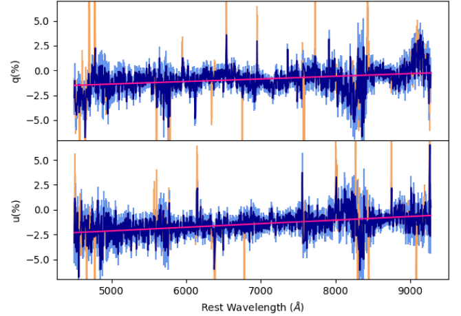
Figure 3. Stokes parameters q and u at +40 days (dark blue; errors in light blue) 3\sigma -clipped according to \Delta\epsilon ; the discarded points are shown in orange. The bin size for the data is 3.3\text{\AA} . The fits to the \sigma -clipped data are shown in magenta.
