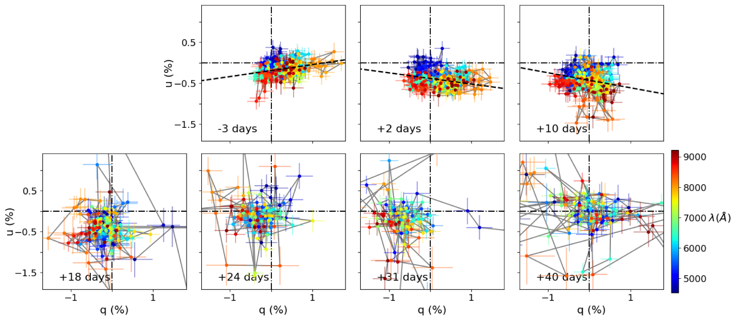
Figure 9. Stokes q-u planes of the ISP corrected data of SN 2011hs from -3 days to 40 days after V-band maximum. The data were binned to 15 \text{ \AA} and the colour scale represents wavelength. The dominant axes of epoch 1 to 3 are shown as the dashed black line, and were calculated using Orthogonal Distance Regression (ODR).
