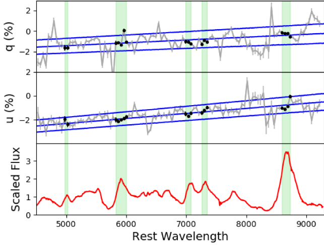
Figure 2. Linear regression (blue) of the Stokes parameters q and u at +40 days in the wavelength range corresponding to emission lines (green highlight). The fitted points are shown in black. The 1\text{-}\sigma lines above and below the fits were determined using Monte Carlo sampling of the gradient and intercept of q_{\text{ISP}} and u_{\text{ISP}} within their errors. The flux spectrum at +40 days is shown in red.
