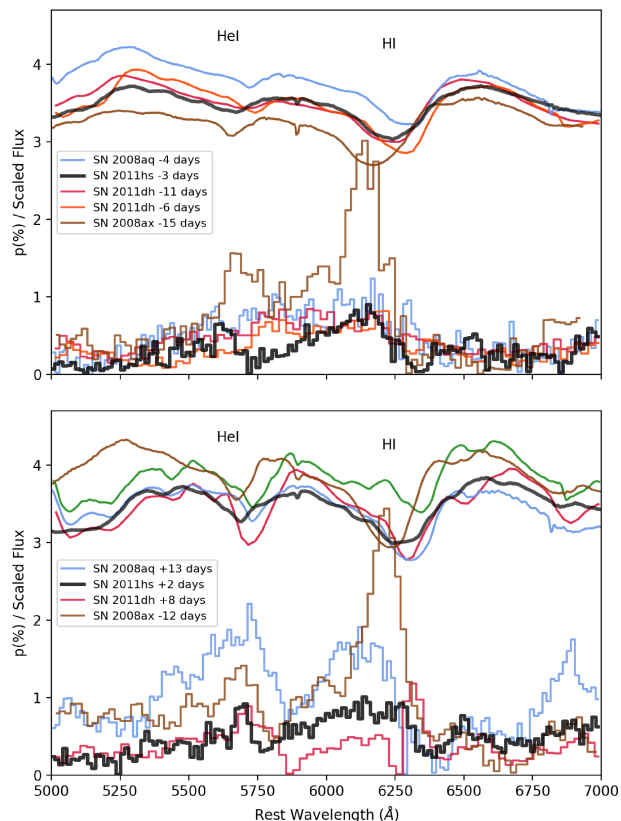
Figure 11. H \alpha and He I \lambda 5876 polarization features in phases where hydrogen dominates (top panel) and after helium has strengthened (bottom panel). We show SN 2011hs, SN 2008ax (Chornock et al. 2011), SN 2011dh (Mauerhan et al. 2015) and SN 2008aq (Stevance et al. 2016). The polarization data are shown as step plots and the flux spectra are plotted for comparison as smooth curves. Note that the phases are quoted with respect to V-band maximum instead of explosion date.
