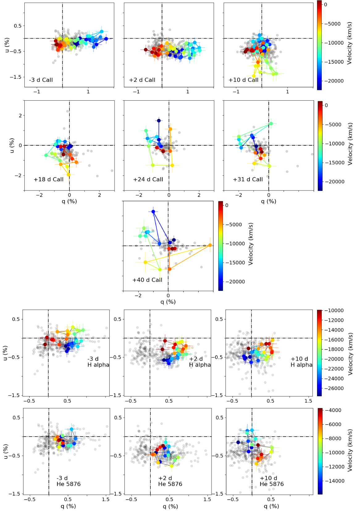
Figure 10. Stokes q-u plots of the ISP corrected data of \text{He } \lambda 5876 and \text{H}\alpha and \text{Ca II} . The colour scales represent velocity in \text{km s}^{-1} and vary between species for better visualisation. The grey points show the rest of the data across the whole wavelength range covered by our observations.
