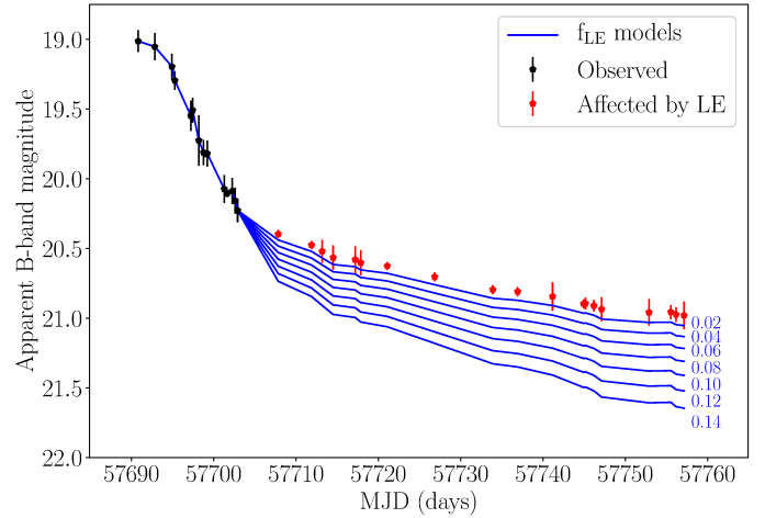
Fig. A.3. Effect of subtracting different fractional contribution of the light-echo to the SN 2016hmk B band observed light curve.
