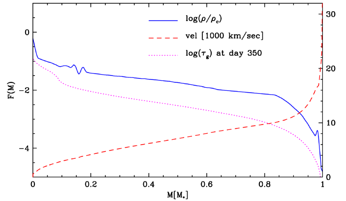
Fig. 24. Structure during the phase of homologous expansion as a function of the mass coordinate in WD-masses for our subluminal model with high central density. We give the normalized density as \log(\rho/\rho_c) (left scale), velocity (right scale) and the mean optical depth \log(\tau_\gamma) (left scale) in \gamma -rays at day 350.
