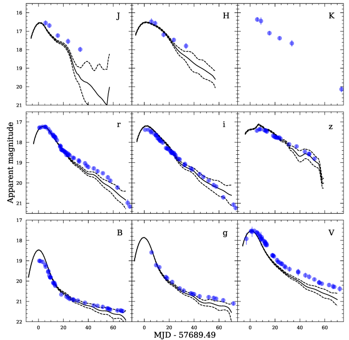
Fig. A.4. Multiband SN 2016hmk SNooPy fits using a 91bg template and with a 10% contribution of a light echo starting at +15 days until the end of the light curve. Fits in all band are reasonably better than those without a LE shown in Figure 7.
