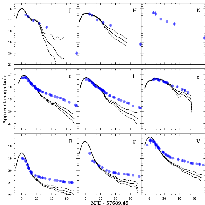
Fig. 7. Multi-band light curves of SN 2016hnk (filled circles) compared with a 1991bg-like template (lines). Best-fit SNOOPy parameters are R_V=2.1 and a host-galaxy color excess of E(B-V)_{\text{host}}=0.55 mag. Note that beyond +20 d the template fit does not succeed in capturing the SN brightness.
