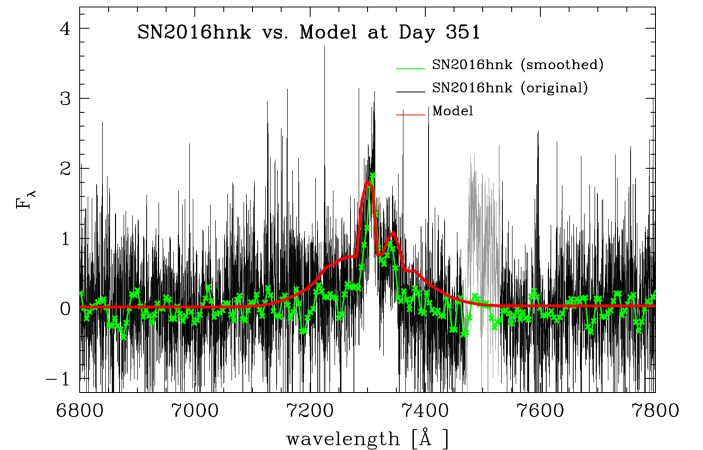
Fig. 27. Comparison of the nebular spectrum of SN 2016hbk with our high-density delayed-detonation model in the rest frame assuming a redshift of z = 0.01610 . The flux is in 10^{-18} \text{ erg s}^{-1} \text{ cm}^{-2} on the same scale as Figure 19. The telluric region in the original spectrum is plotted in gray, around 7,500 \text{ \AA} . The theoretical spectrum is dominated by a narrow, forbidden [Ca II] doublet at 7291 and 7324 \text{ \AA} above a quasi-continuum at about the 3% level formed by many transitions of mostly heavier elements including Fe, Co, Ni, Cr, etc.
