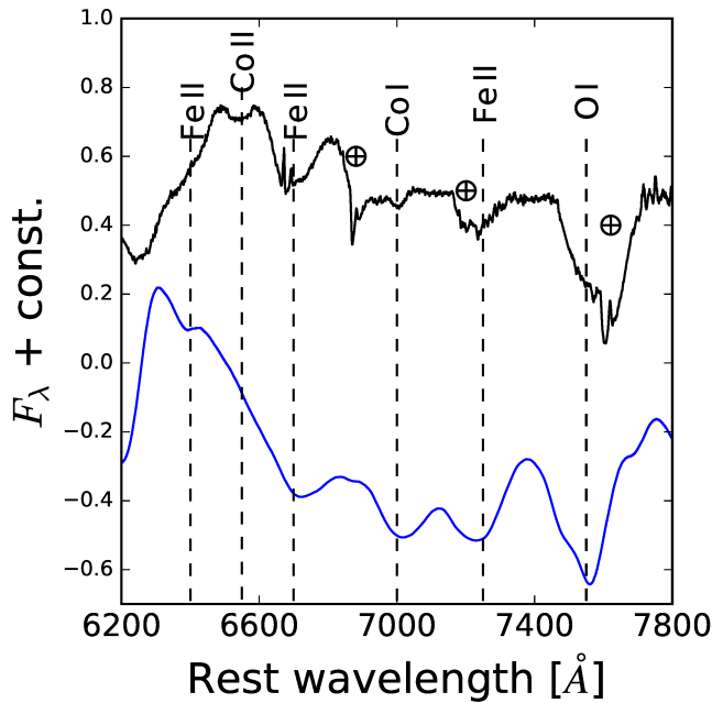
Fig. 22. Comparison of SN 2016hmk (black) +2.5 d past maximum light and the non-LTE model of SN 1999by at +7 days past maximum light (blue) from Höflich et al. (2002). The telluric features are marked in the observed spectra.
