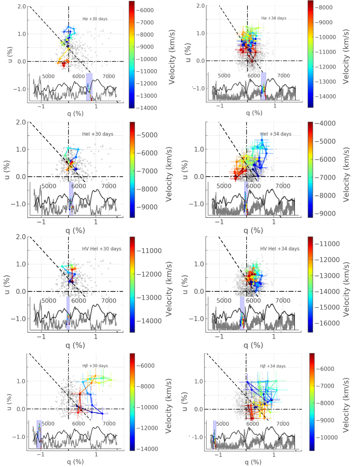
Figure 10. ISP corrected H \beta , H \alpha and HeI \lambda 5876 polarization of SN 1993J on April 26 (+30 days) and April 30 (+34 days). The colour bars represent velocity. The inset plots show the flux spectrum in dark grey and the polarization in light grey. The data points shown on the q-u plots are presented with the corresponding colour map and highlighted by the shaded blue region. The dashed line indicates the direction of the dominant axis as reported in Table 4.
