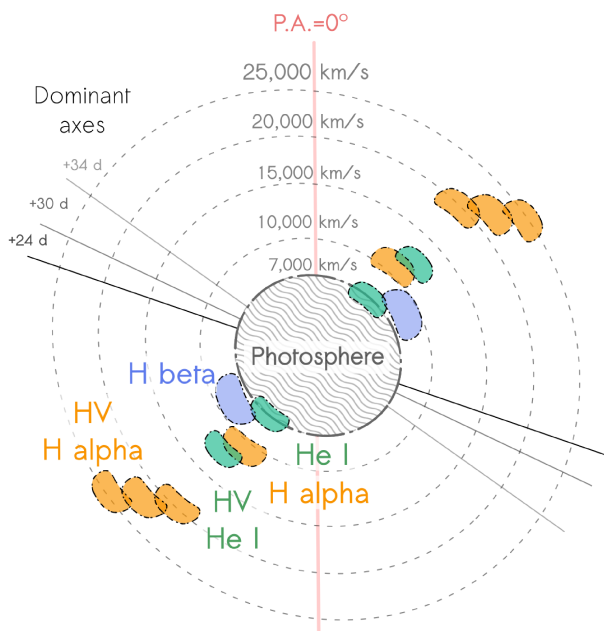
Figure 12. Visualisation of the features of SN 1993J based on our first three epochs of spectropolarimetric data. The details of how this illustration was built are given in Section 5.3 - we note that since Stokes parameters are pseudo-vectors, unavoidable artificial symmetry is introduced. The figure shows the SN projected onto the plane of the sky. However, the clumps are rotated through -90^\circ and +90^\circ , respectively, about the symmetry axis of the epoch of each observation to indicate their velocities. In reality, the absorption character of the corresponding spectral features implies that the clumps are located between the photosphere and the observer.
