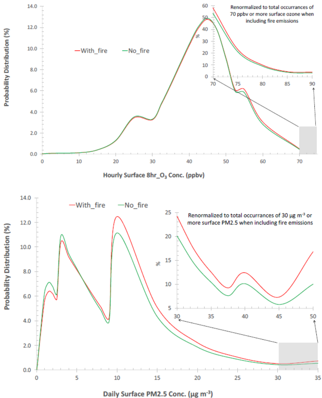
Figure 7. Probability distribution of surface 8-hr average \text{O}_3 (top) and 24-hr average \text{PM}_{2.5} (bottom) concentrations over the contiguous U.S. The inset on each plot is the re-normalized probability distribution of the corresponding pollutant at tail with high concentrations.
