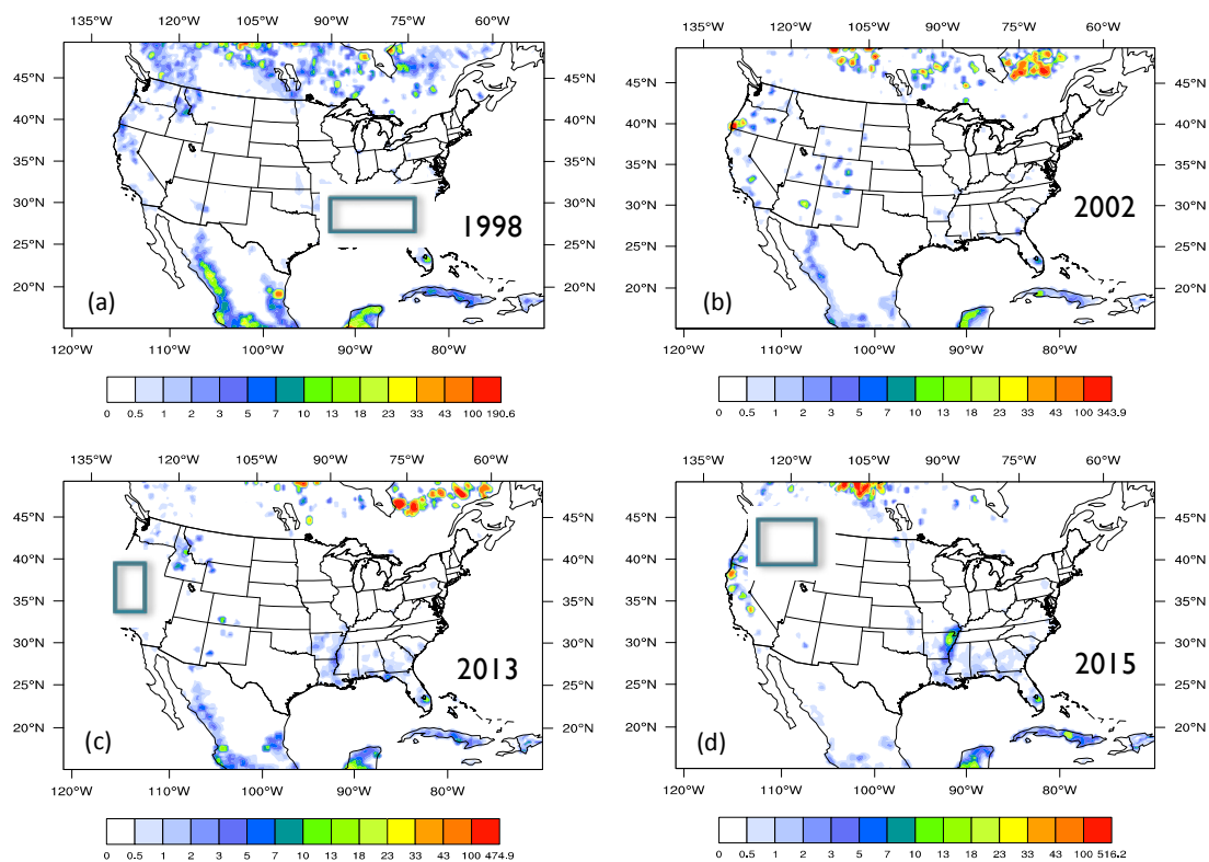
Figure 2. Spatial distributions of fire CO emissions ( \text{tons km}^{-2} \text{yr}^{-1} ) for 1998, 2002, 2013, and 2015. Boxes over the maps represent the sub-regions subject to further analysis—southeastern U.S.; Northern California, and northwestern U.S.
