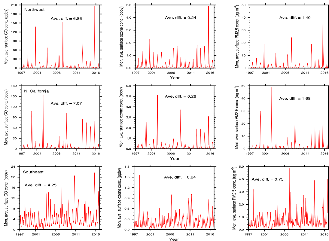
Figure 6. Evolutions of fire contributions to monthly average surface CO (ppbv), O 3 (ppbv), and PM 2.5 (µg m -3 ) for the northwestern U.S., Northern California, and the southeastern U.S. from 1997 to 2016.
