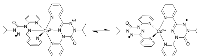
Scheme 2. Valence tautomeric equilibrium in [\text{Co}(\text{dipyvd})_2]^{2+} .
