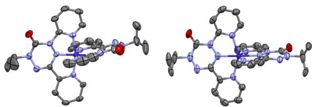
Figure 2. Thermal ellipsoid plots of the cation in [\text{Co}(\text{dipyvd})_2]^{2+}(\text{PF}_6^-) (left) and [\text{Co}(\text{dipyvd})_2]^{2+}(\text{PF}_6^-)_2 (right). Ellipsoids are drawn at the 50% level. Hydrogen atoms have been omitted for clarity
