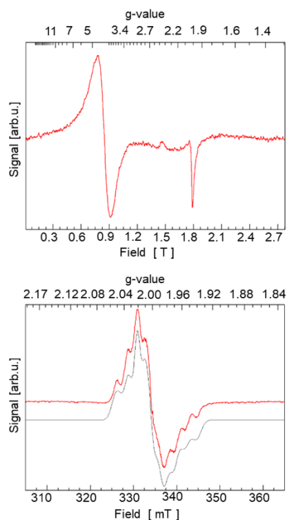
Figure 4. CW EPR spectra recorded for [\text{Co}(\text{dipyvd})_2](\text{PF}_6)_2 . Top: Spectrum recorded at 5 K and 50.3 GHz for a neat powder sample of [\text{Co}(\text{dipyvd})_2](\text{PF}_6)_2 . Bottom: X-band EPR spectrum recorded at 77 K for a MeCN solution of [\text{Co}(\text{dipyvd})_2](\text{PF}_6)_2 . The experimental spectrum shown in red was recorded using a microwave frequency of 9.36 GHz, modulation amplitude of 3 G, modulation frequency of 100 kHz, and microwave power of 2 mW. Shown in black is a simulation obtained for a S = 1/2 and I = 7/2 such that g_x = 1.988 , g_y = 1.994 , g_z = 2.011 , \sigma(g_x) = 0.009 , \sigma(g_y) = 0.005 , \sigma(g_z) = 0.001 , A_x = 8.42 MHz, A_y = 75 MHz, A_z = 10.46 MHz, and an intrinsic linewidth of 6 G.
