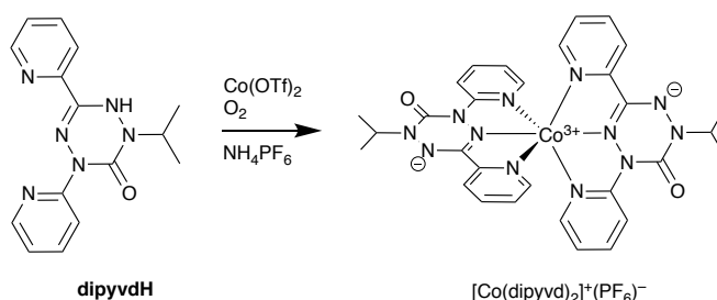
Scheme 1. Synthesis of [Co(dipyvd)_2](PF_6)_2
