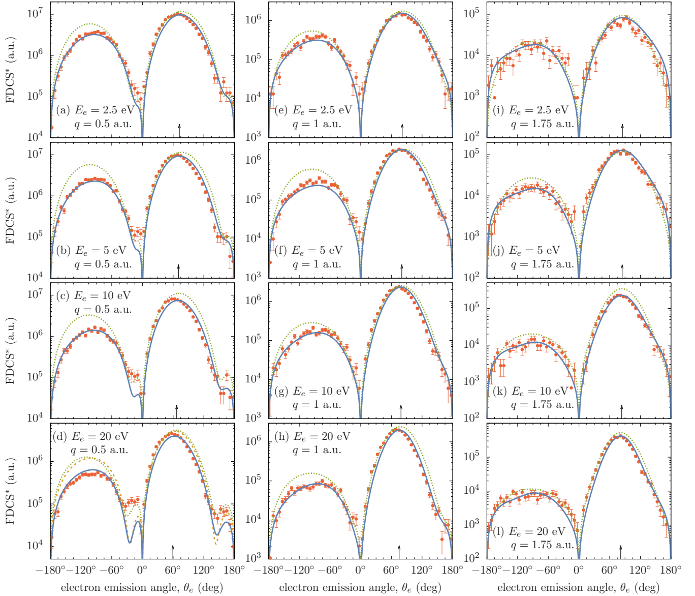
FIG. 1. Fully differential cross sections (FDCS*) for single ionization of helium by 1-MeV protons in the scattering plane ( \phi_e = 0^\circ ) as a function of the polar angle of the ejected electron for the electron emission energies and momentum transfers indicated in the legend. The present WP-CCC predictions (shown by blue solid lines) are compared with the experimental data (red dots with error bars), FBA (green dotted lines), and 3C (brown dashed lines) calculations by Chuluunbaatar et al. [27]. The FBA results of Chuluunbaatar et al. [27] are convolved with the experimental uncertainties in ejected energy \Delta E_e and momentum transfer \Delta q . The arrow in each panel indicates the direction of the momentum transfer.
