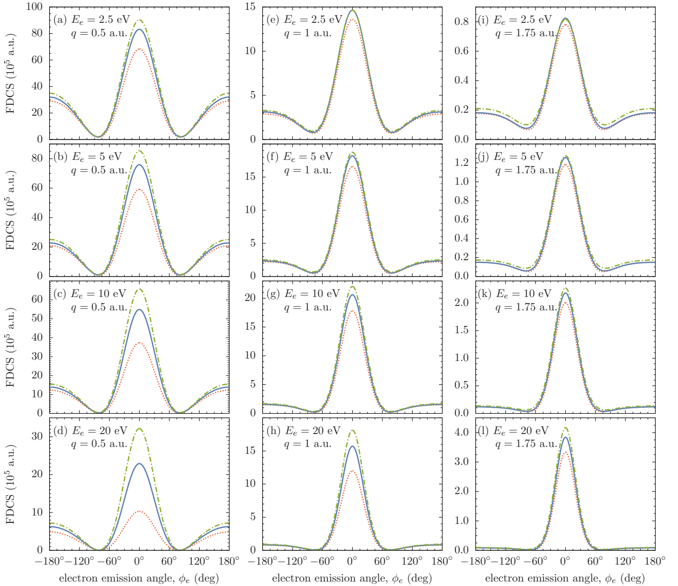
FIG. 4. WP-CCC results for the fully differential cross sections for single ionization of helium by 500-keV (red dotted lines), 1-MeV (blue solid lines), and 2-MeV (green dot-dashed lines) protons in the azimuthal plane ( \theta_e = 90^\circ ) as a function of the azimuthal angle of the ejected electron for the electron emission energies and momentum transfers indicated in the legend.
