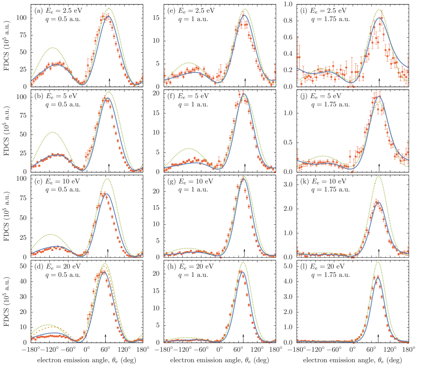
FIG. 2. Fully differential cross sections (FDCS) for single ionization of helium by 1-MeV protons in the scattering plane ( \phi_e = 0^\circ ) as a function of the polar angle of the ejected electron for the electron emission energies and momentum transfers indicated in the legend. The present WP-CCC predictions (shown by blue solid lines) are compared with the experimental data (red dots with error bars), FBA (green dotted lines), and 3C (brown dashed lines) calculations by Chuluunbaatar et al. [27]. The FBA results of Chuluunbaatar et al. [27] are convolved with the experimental uncertainties in ejected energy \Delta E_e and momentum transfer \Delta q . The arrow in each panel indicates the direction of the momentum transfer.
