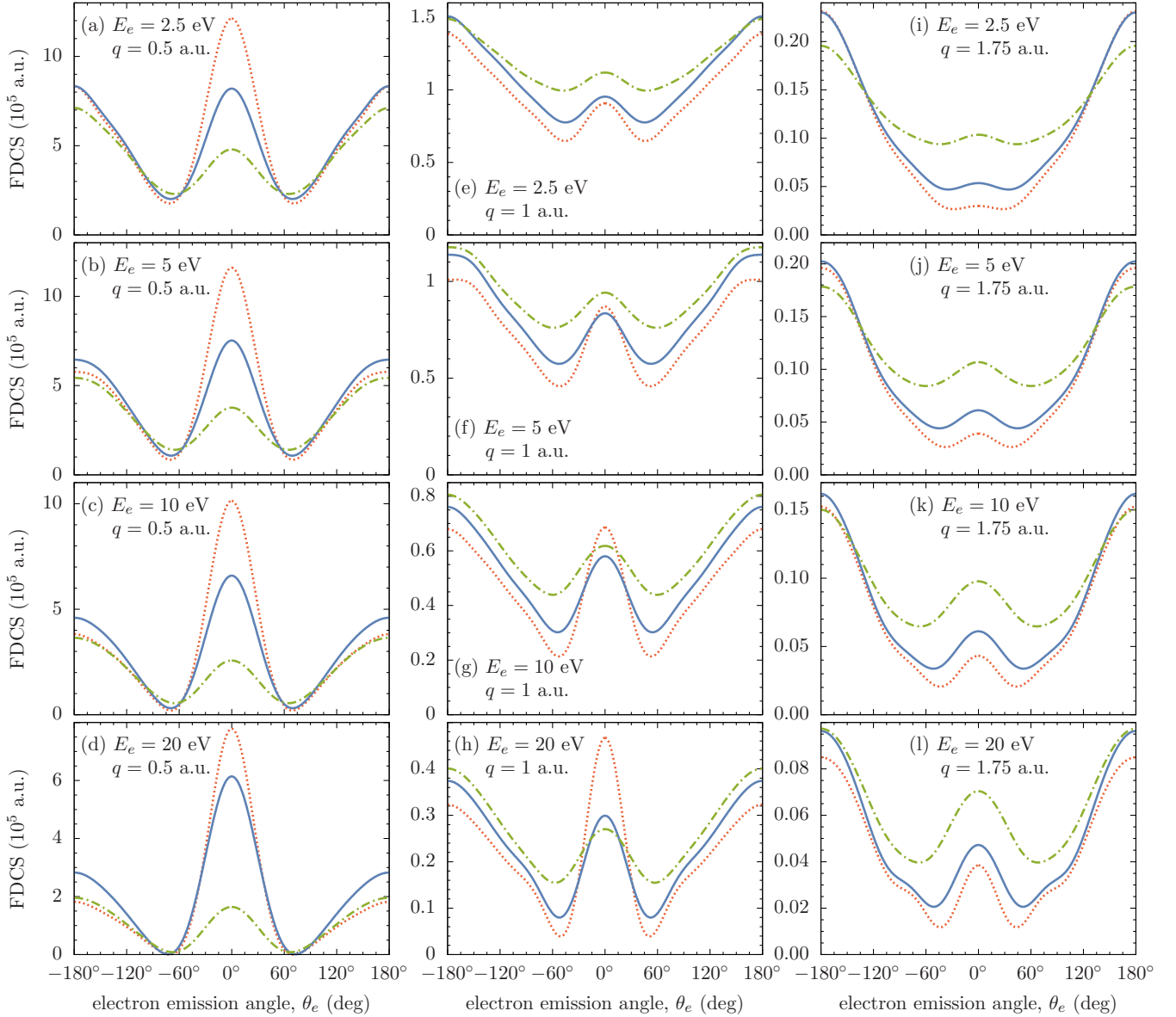
FIG. 5. WP-CCC calculations for the fully differential cross sections for single ionization of helium by 500-keV (red dotted lines), 1-MeV (blue solid lines), and 2-MeV (green dot-dashed lines) protons in the perpendicular plane ( \phi_e = 90^\circ ) as a function of the polar angle of the ejected electron for the electron emission energies and momentum transfers indicated in the legend.
