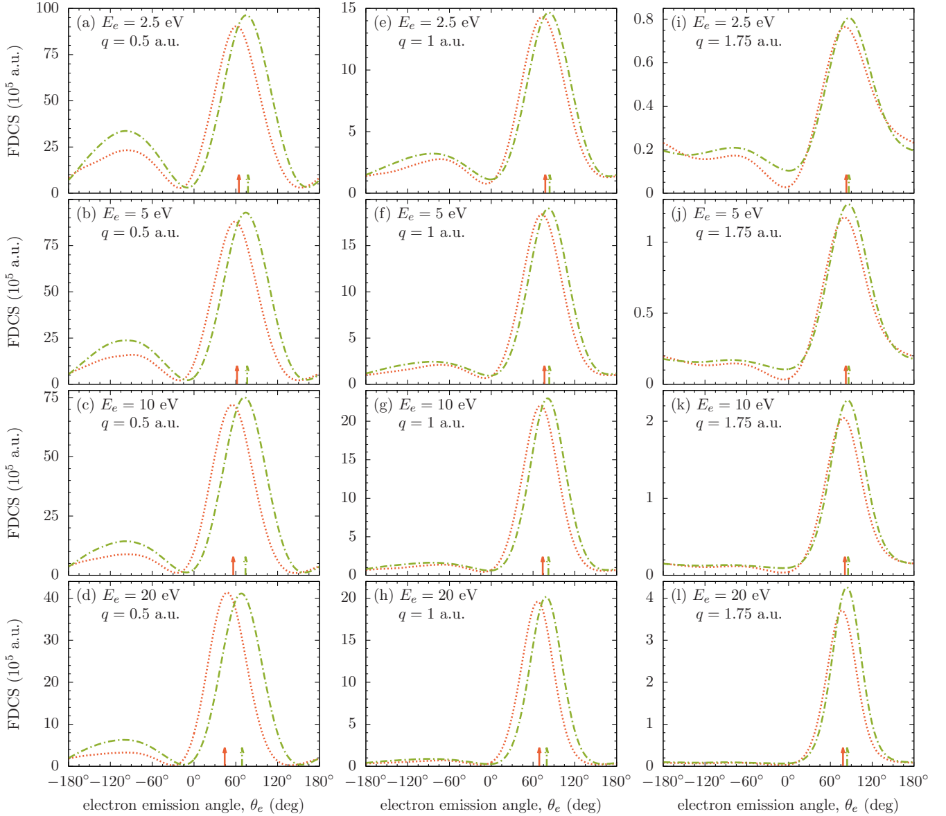
FIG. 3. WP-CCC calculations for the fully differential cross sections for single ionization of helium by 500-keV (red dotted lines) and 2-MeV (green dot-dashed lines) protons in the scattering plane ( \phi_e = 0^\circ ) as a function of the polar angle of the ejected electron for the electron emission energies and momentum transfers indicated in the legend. The arrow in each panel indicates the direction of the momentum transfer.
