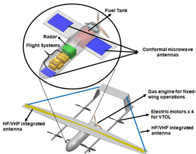
Fig. 12. Fixed-wing VTOL platform with integrated antennas.
