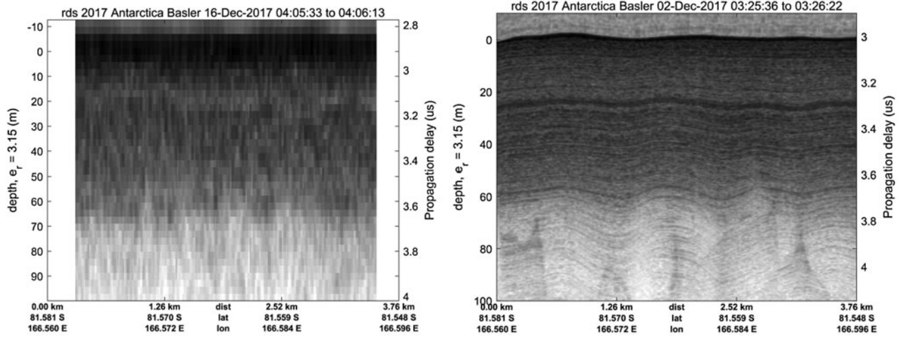
Fig. 3. Echogram from the UWB RDS/I system on the Airtac Basler. Narrowband data (left) and wideband data from two cross-over lines over Ross Ice Shelf Antarctica. These echograms show the first 100 m below the surface, and the improvement in internal layer detection of the wideband operation is apparent.
