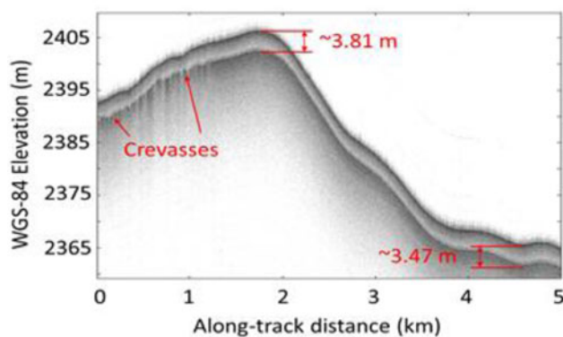
Fig. 10. Measured seasonal snow depth over Walsh Glacier (left), and radar echogram showing multiple snow layers over Chisana Glacier (right) (Li and others, 2019c). These data were collected using the Snow-C installed on the Single Otter.
