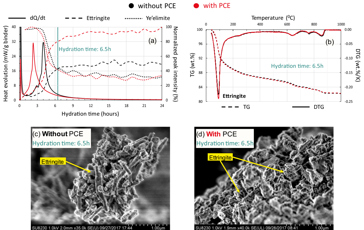
Fig. 10. Influence of PCE on (a) hydration kinetics, (b) phase development and (c, d) phase morphology in CSA paste mixtures.
