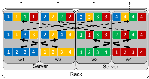
Figure 10: An example hierarchical transfer. Each worker groups its tuples by partition key, and sends them first within a server, then within a rack, and finally to their destinations. A naïve system would send directly to other racks. Colors track where the tuple was generated; numbers indicate the partition.
