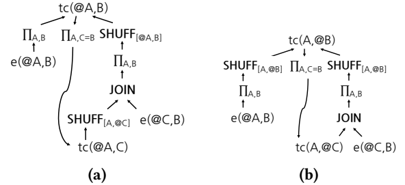
Figure 8: Two potential partitionings for TC.
