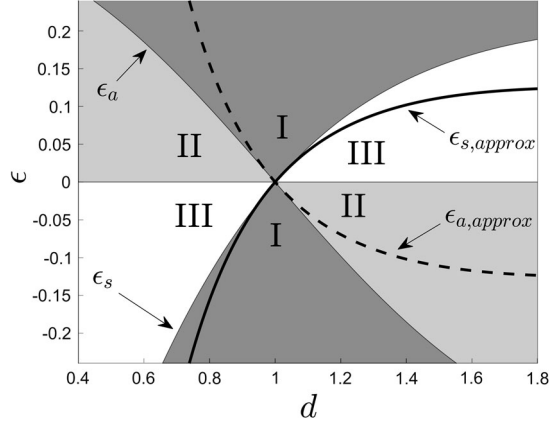
FIG. 1. Above, the intersection of \epsilon_a and \epsilon_s as given by (9) define regions for which locking (either synchronous or antiphase) is stable for the CGL model (7) when q = 1 and (d, \epsilon) vary. Synchrony is only stable in regions I, II; antiphase is only stable in I, III. Thick solid and dashed lines show \epsilon_{s,approx} and \epsilon_{a,approx} , respectively, determined from the higher order phase approximation.
