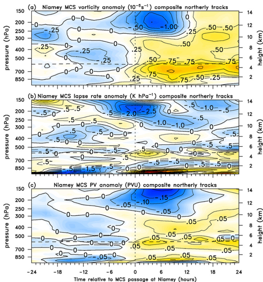
FIG. 16. Time series relative to composite convective line passage of anomalies of (a) vorticity ( 10^{-5} \text{ s}^{-1} ), (b) lapse rate ( \text{K hPa}^{-1} ), and (c) potential vorticity ( \text{PVU} = 10^{-6} \text{ K m}^2 \text{ kg}^{-1} \text{ s}^{-1} ) at Niamey radar site. Anomalies are relative to the monsoon period (10 Jul–15 Sep) mean fields. Horizontal dashed lines denote 0^\circ\text{C} level.
