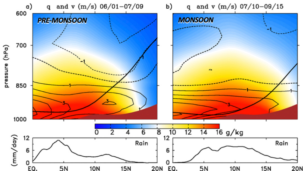
FIG. 6. North–south cross sections ( 0^\circ – 20^\circ\text{N} ) averaged from 0^\circ to 7^\circ\text{E} of (a) premonsoon and (b) monsoon meridional wind v ( \text{m s}^{-1} , contours) and specific humidity q ( \text{g kg}^{-1} , color). TRMM rainfall is shown at bottom. Heavy solid lines are estimates of cloud-base height based on surface observations. Cloud-base height (CBH) in km is computed as \text{CBH} = 0.125(T_s - T_d) from Stull (1988), where T_s is the surface temperature and T_d is the surface dewpoint temperature. Dark brown shaded areas denote topography.
