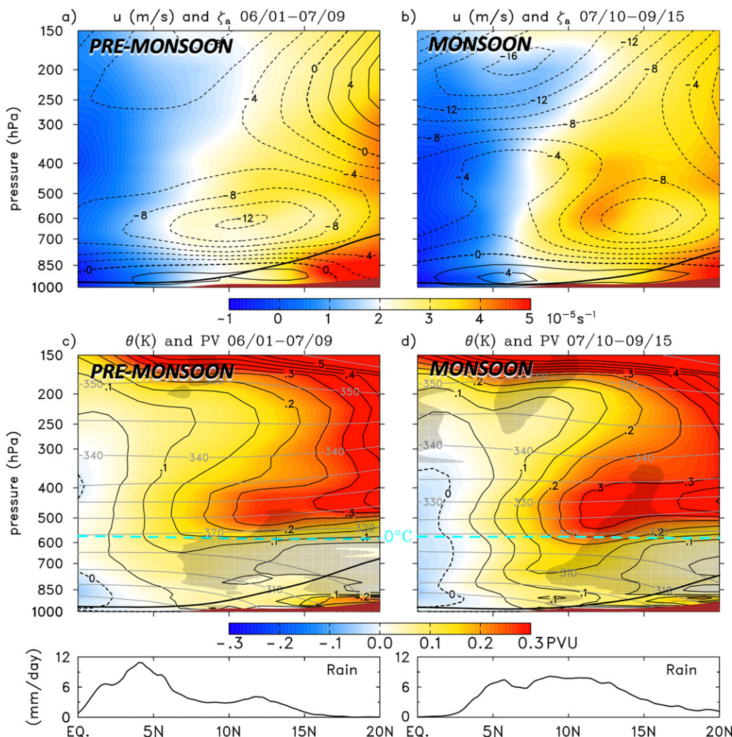
FIG. 7. North-south cross sections ( 0^\circ – 20^\circ\text{N} ) averaged from 0^\circ to 7^\circ\text{E} of (a) premonsoon and (b) monsoon zonal wind ( \text{m s}^{-1} , contours) and absolute vorticity \zeta_a ( 10^{-5} \text{ s}^{-1} , color), and (c) premonsoon and (d) monsoon potential vorticity PV ( \text{PVU} = 10^{-6} \text{ K m}^2 \text{ kg}^{-1} \text{ s}^{-1} , contoured colors) and potential temperature (K, gray solid contours). Stippled areas in (c) and (d) indicate where the north-south gradient of PV is negative. TRMM rainfall is shown at bottom. Heavy solid lines are estimates of cloud-base height based on surface observations. Dashed light blue line denotes 0^\circ\text{C} level.
