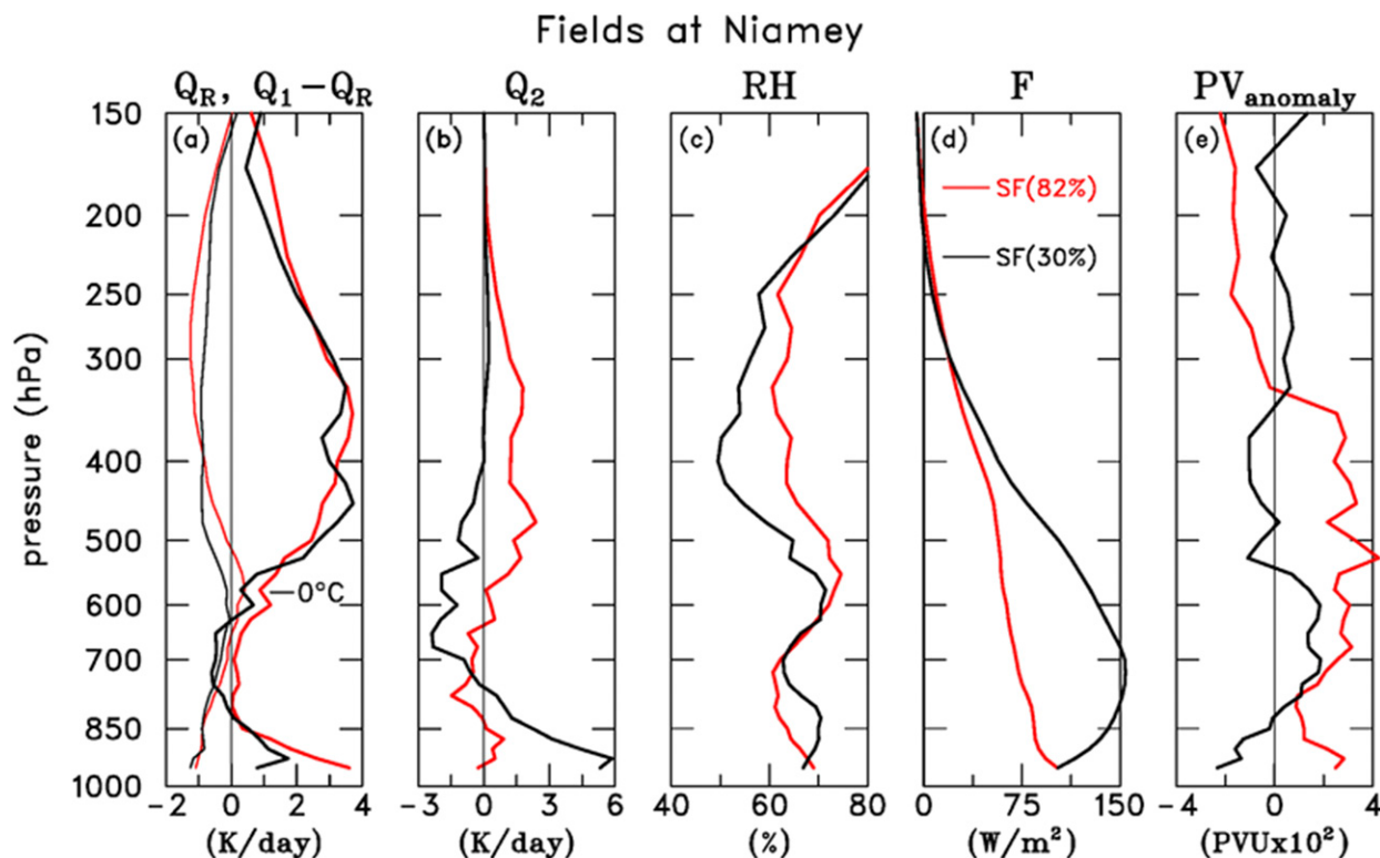
FIG. 9. Vertical profiles of (a) radiative heating rate Q_R (thin curves) and convective heat source Q_1 - Q_R (thick curves) in units of \text{K day}^{-1} , (b) apparent moisture sink Q_2 ( \text{K day}^{-1} ), (c) relative humidity (%), with respect to ice for subfreezing temperatures), (d) vertical eddy flux of moist static energy F ( \text{W m}^{-2} ), and (e) potential vorticity anomaly ( \text{PVU} = 10^{-6} \text{ K m}^2 \text{ kg}^{-1} \text{ s}^{-1} ) for MIT-radar-based average stratiform fraction SF of 82% (red) and 30% (black). In other words, the red (black) curves can be considered representative of precipitation events predominantly stratiform (convective) in nature. Curves show profiles when radar times matched up with sonde times during the period when radar data were available.
