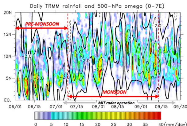
FIG. 5. June–September 2006 TRMM 3B42 rainfall (color; \text{mm day}^{-1} ) from 0^\circ to 20^\circ\text{N} over longitudes of sounding arrays ( 0^\circ – 7^\circ\text{E} ) overlain by 500-hPa vertical p velocity (contours; \text{hPa h}^{-1} ) for the period of the special AMMA sounding operations. Premonsoon period is defined as 1 Jun–9 Jul, monsoon period 10 Jul–15 Sep. Period of MIT radar operation indicated by gray arrows.
