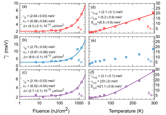
FIG. 3. Fluence and temperature dependence of the exciton dephasing rates. Dephasing parameters \gamma of excitons A, A', and B [panels (a) and (d), (b) and (e), and (c) and (f), respectively] obtained from the simultaneous fitting of diagonal and anti-diagonal cuts, plotted as a function of excitation fluence [panels (a)–(c)] or temperature [panels (d)–(f)]. Squares represent the experimental linewidths and lines are the best fit to the relevant model described in the main text. Error bars on the data are contained within the markers. For panels (a)–(c), the sample's temperature is maintained at 5 K while the excitation fluence is kept at 50 \text{nJ/cm}^2 for measurements presented in panels (d)–(f).
