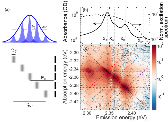
FIG. 1. Linear and two-dimensional coherent spectroscopy of (\text{PEA})_2\text{PbI}_4 at 5 K. (a) Illustration of the inhomogeneous and homogeneous nature of line broadening. The total linewidth (blue line) is composed of a distribution of homogeneously broadened lines (blue areas). This arises from the simultaneous existence of uncorrelated transitions from the ground state (black lines) to short-lived excited states (blurred lines). E_0 represents the central energy, and \delta\omega and 2\gamma are the inhomogeneous and homogeneous linewidths respectively. (b) Absorption spectrum of (\text{PEA})_2\text{PbI}_4 measured at 5 K (black line) and normalized spectrum of the pulses used in 2D coherent excitation spectroscopy measurements (dashed line). Both scales are logarithmic. Dotted lines indicate the energy of excitons A, A', B, and B*, respectively, with increasing energy. (c) Absolute value of the 2D coherent rephasing spectrum of (\text{PEA})_2\text{PbI}_4 measured at 5 K with a pulse fluence of 40 \text{ nJ/cm}^2 and a pump-probe delay of 20 fs. The color scale is logarithmic. Dotted lines indicate the energies of the aforementioned features. The paths of the diagonal cut (black dashed line) and antidiagonal cuts at the diagonal energy of excitons A, A', and B (red, blue, and purple dashed lines, respectively) are also shown.
