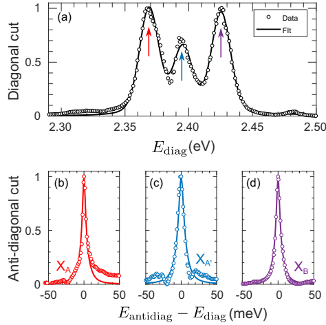
FIG. 2. Fitting diagonal and anti-diagonal spectral cuts to a line-shape model. Normalized diagonal cut (a) and anti-diagonal cuts at diagonal energies of excitons A, A', and B [panels (b)–(d), respectively] of the two-dimensional coherent excitation rephasing spectrum presented in Fig. 1(c) (circles) and the result of the fitting procedure described in the main text (lines). Arrows in panel (a) mark the position along the diagonal where the anti-diagonal cuts cross it. Because of the presence of low-amplitude cross peaks in the 2D spectrum, these also appear in the tails of the anti-diagonal cuts. To minimize their effect on the quality of the fits and to avoid overestimation of the linewidths, only points higher than 15% of an anti-diagonal cut maxima were included in the fit. The quality of the fits presented here are representative of all the presented dataset. To test the robustness of the fits and to estimate the uncertainties on the extracted linewidths, we repeated the fitting procedure numerous times while adding white noise (5% of the cut's maximum peak to the data).
