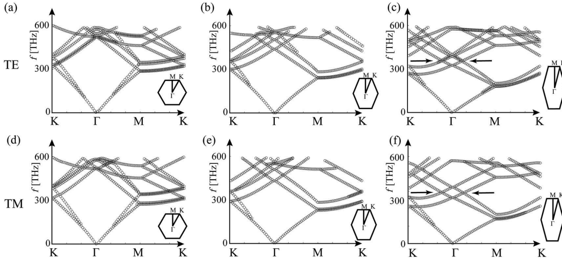
Fig. 3 Numerical simulation results presenting the bandstructure of photonic slab WG modes (i.e., frequency as a function of the corresponding directions in the k -space) formed in a suspended photonic liquid lattice of hexagonal symmetry and hexagonal broken symmetry. (a)–(c) Bandstructure of TE slab WG modes in a suspended photonic liquid lattice presented in Figs. 1(b)–1(d) due to interference formed by three plane waves at angles (a) \theta = \pi/6 , (b) \pi/4 , and (c) \pi/3 . (d)–(f) Bandstructure of TM slab WG modes at interference angles (d) \theta = \pi/6 , (e) \pi/4 , and (f) \pi/3 . Two Dirac points emerge at the angle \theta = \pi/3 at frequencies around 353 and 349 THz, respectively, marked at (c) and (f) by black arrows. In the simulation, the refractive index is 1.409, the mean TLD film thickness is 450 nm, and the peak-to-peak undulation amplitude is 300 nm.
