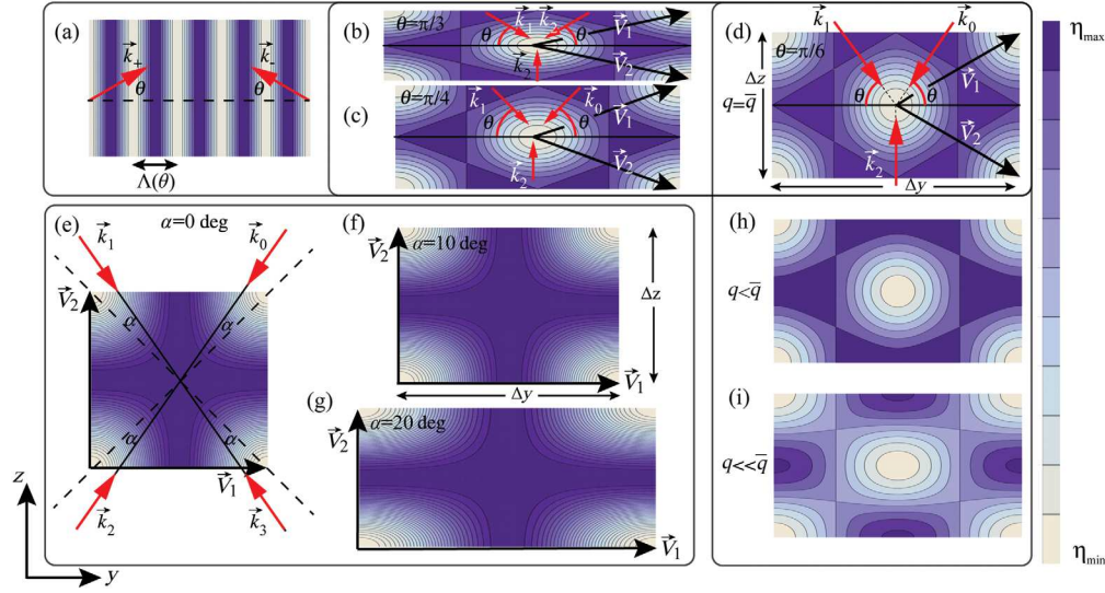
Fig. 2 Optical liquid lattices formed from a TLD film due to interference of SPPs or WG plane wave modes with propagating direction marked with red arrows. (a) One-dimensional lattice formed by interference of two surface optical plane waves with \theta -dependent periodicity given by Eq. (6). (b)–(d) Two-dimensional lattices of hexagonal symmetry and (e)–(g) rectangular symmetry, where \vec{V}_1 and \vec{V}_2 are the corresponding primitive vectors. The symmetry of the liquid lattice and can be controlled by the relative angles of the interfering beams; (b) \theta = 30^\circ and (c) \theta = 45^\circ are lattices with hexagonal broken/distorted symmetry, whereas (d) \theta = 60^\circ is hexagonal symmetric lattice; (e) \alpha = 0^\circ (square symmetry), (f) \alpha = 10^\circ , and (g) \alpha = 20^\circ correspond to rectangular symmetry. (h), (i) Optical liquid lattice for different values of q which results in (d) a phase transition from a hexagonal lattice to (h) merging of the triangular sites and (i) face-centered cubic lattice. The 2-D liquid lattices are normalized by \eta_{\max} and \eta_{\min} \equiv -\eta_{\max} defined in Eq. (9) and below Eq. (11).
