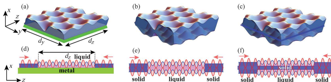
Fig. 1 Schematic presentation of TLD film deformation forming optical liquid lattices (blue) due to surface tension effects triggered by interference of surface optical modes (red). (a) 2-D plasmonic liquid lattice formed by interference of SPPs. (b), (c) Suspended and supported photonic liquid lattice, respectively, formed by interference of photonic slab WG modes. Gain can be introduced into the suspended structure (c) either to the liquid or to the dielectric supporting membrane. The lateral dimensions of the liquid slots, which are bounded by solid dielectric walls (not shown) are d_y and d_z . (d)–(f) The corresponding 1-D optical liquid lattices in a liquid slot of length d_z induced by pairs of (d) counterpropagating SPPs or (e) and (f) slab WG modes.
