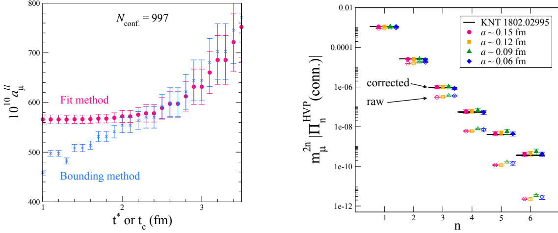
Figure 1: Left: Values of a_\mu^H obtained with different methods for handling the high t contribution, namely, our “fit method” and the BMW “bounding method” [10]. They agree well for t > 2.3 fm. Right: Raw (open symbols) and corrected (filled symbols) vacuum-polarization Taylor coefficients. They agree well with results from the R-ratio method, shown with black lines [3].
