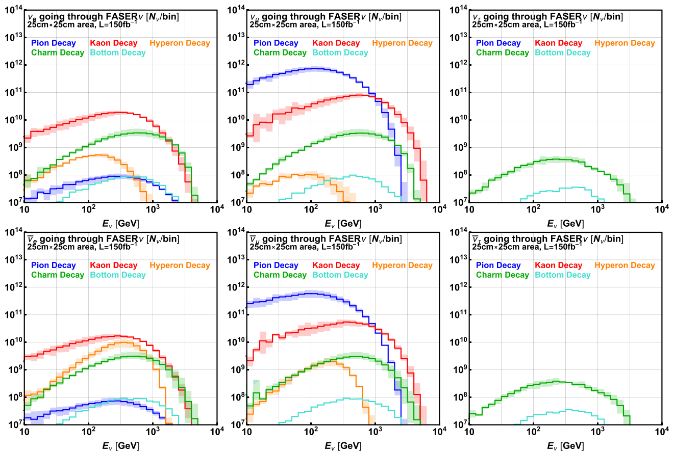
Fig. 4 The estimated number of neutrinos that pass through the 25\text{ cm} \times 25\text{ cm} transverse area of FASER \nu , assuming an integrated luminosity of 150\text{ fb}^{-1} for Run 3 at the 14 TeV LHC. The event rates are for electron (left), muon (center), and tau (right) neutrinos (upper)
