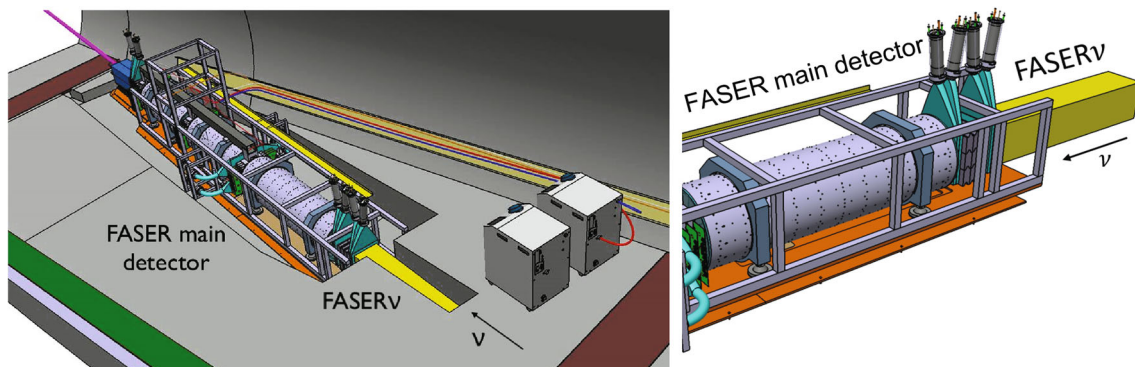
Fig. 2 View of FASER, including the FASER \nu detector, in tunnel TI12, 480 m downstream from the ATLAS IP along the beam collision axis. The FASER \nu detector is a 25\text{ cm} \times 25\text{ cm} \times 1.35\text{ m} emulsion detector, consisting of 1000 layers of emulsion films interleaved with
