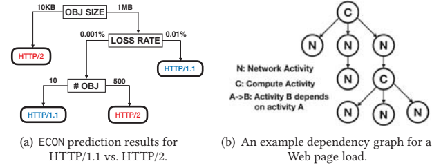
Figure 11: Decision tree and Web dependency graph.
