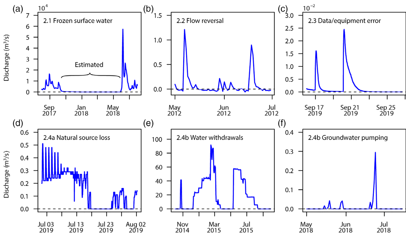
FIGURE 3 Examples of daily hydrographs displaying zero-flow readings. (a) Kugaruk River, near Deadhorse, AK (USGS site: 15896000), (b) Berger Ditch near Oregon, OH (USGS site: 04194085), (c) Rio Puerco near Bernardo, NM (USGS site: 08353000, provisional data downloaded September 26, 2019), (d) Agua Fria River Near Mayer, AZ (USGS site: 09512500, provisional data downloaded Sep. 26, 2019), (e) Snake River near Milner Dam, ID (non-USGS gage), and (f) Arkansas River at Garden City, KS (USGS site: 07139000). Subplot subtitles indicate the associated zero-flow scenarios as illustrated in Figure 2. Data source: U.S. Geological Survey, 2019
