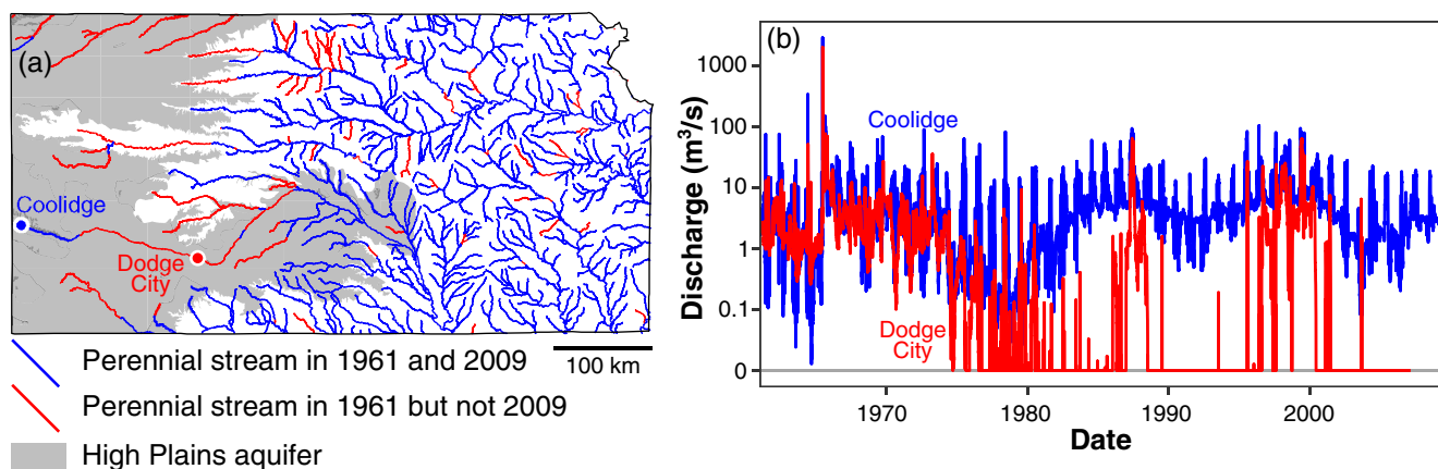
FIGURE 5 (a) Map of Kansas (United States) showing regional transitions from perennial to non-perennial flow between 1961 and 2009 resulting from groundwater pumping from the High Plains aquifer. (b) Time series of discharge (1961–2009) from Arkansas River at Coolidge, KS (USGS gage 07137500) and Arkansas River at Dodge City, KS (USGS gage 07139500) showing increase in zero-flow occurrences through time associated with groundwater depletion between Coolidge and Dodge City. Points in (a) indicate locations of gaging stations plotted in (b). Perennial/non-perennial stream map modified from data used in Kansas High Plains Atlas ( http://www.kgs.ku.edu/HighPlains/HPA_Atlas/index.html ) and based on data collected and interpreted from Kansas Surface Water Register (Kansas Department of Health and Environment, 2013)
