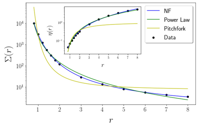
FIG. 5. Comparison of the best fit of \Sigma(w) and \eta(w) derived with different functional forms of \frac{dw}{dr} . We have w = (r - r_c)/s_s such that \Sigma(r) = \Sigma(w) and \eta(r) = \eta(w) . “NF” corresponds to \Sigma and \eta derived from the transcritical normal form, “Power Law” the hyperbolic (power-law) form, and “Pitchfork” the pitchfork form.
