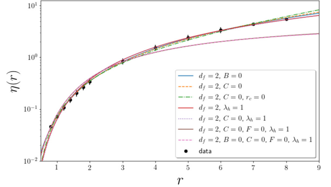
FIG. 10. Fit comparisons \eta(w) for the alternative transcritical form.
