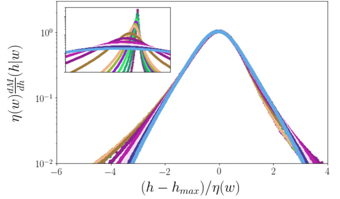
FIG. 4. Scaling collapse of the change in magnetization of the sample with respect to the field \frac{dM}{dh}(h|w) for values of w ranging from 0.8 to 8.0. Again, the shape of this curve is universal.
