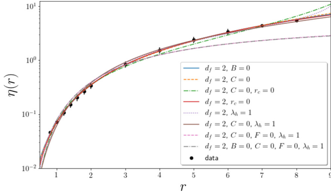
FIG. 8. Fit comparisons \eta(w) for the transcritical form.
