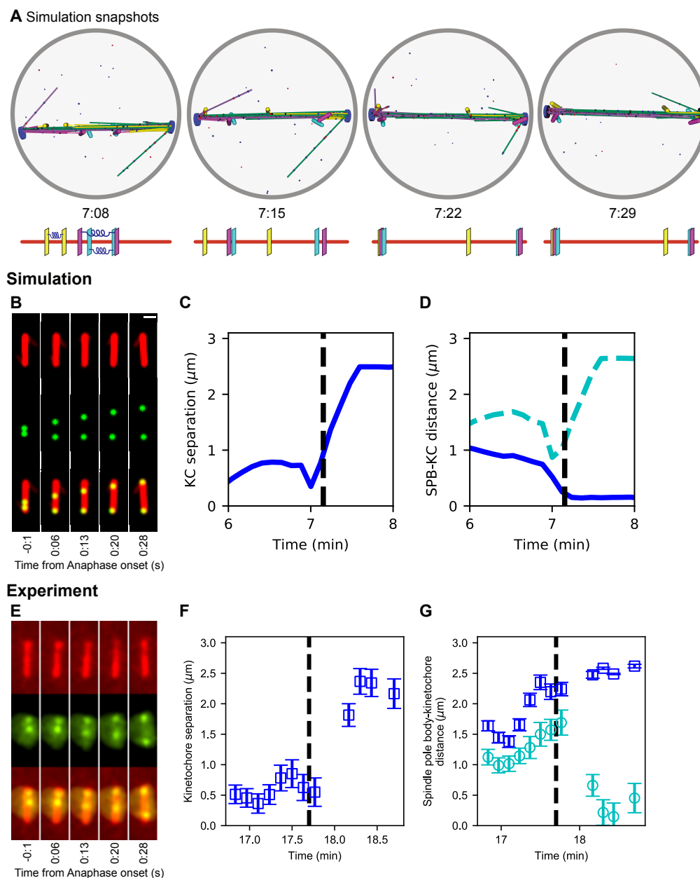
Figure 8: Chromosome segregation in the model and comparison to experiments. (A) Image sequence of simulation of chromosome segregation after anaphase is triggered, rendered from a three-dimensional simulation. Anaphase begins immediately after the first image. Lower, schematic showing kinetochore position along the spindle. Time shown in minutes:seconds. (B-D) Simulation results. (B) Simulated fluorescence microscopy images with MTs (red) and a single kinetochore pair (green). Time shown in minutes:seconds. (C) Spindle pole body-kinetochore distance, and (D) interkinetochore distance versus time from the simulation shown in (B), sampled at a rate comparable to the experimental data in (E-G). (E-G) Experimental results. Maximum-intensity projected smoothed images from time-lapse confocal fluorescence microscopy of fission yeast with mCherry-atb2 labeling MTs (red) and cen2-GFP labeling the centromere of chromosome 2 (green). Time shown in minutes:seconds. (E) Spindle length, (F) spindle pole body-kinetochore distance, and (G) interkinetochore distance versus time from the experiment shown in (E).
