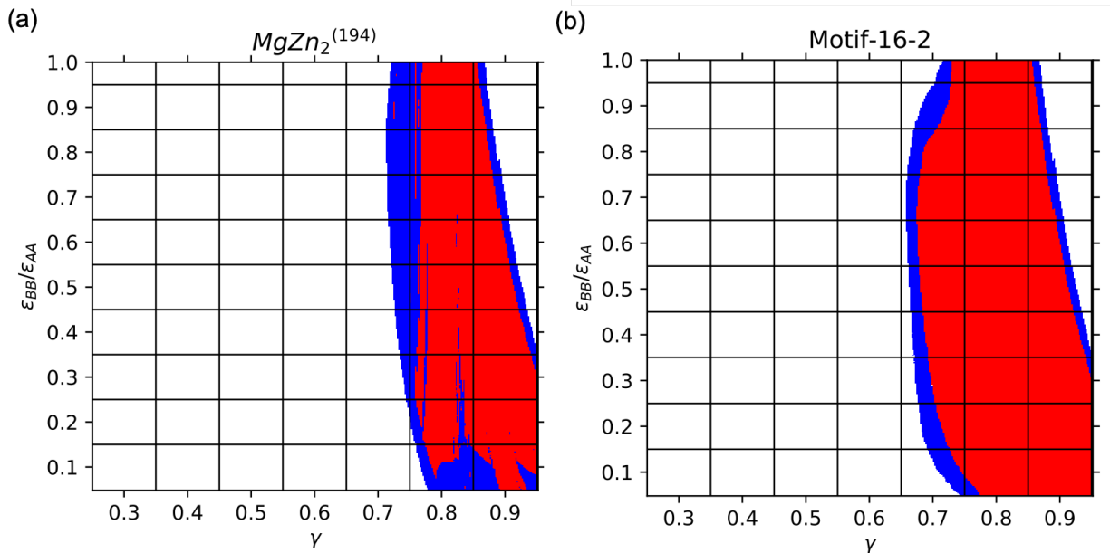
Figure 4: (a) Map of \text{MgZn}_2 in \gamma and \epsilon_{BB} . The red regime indicates that the structure of \text{MgZn}_2 is thermodynamically stable while in blue regime it is metastable. (b) Map for the Z_{16} motif with red stable, blue metastable. The red regime is where the stable structure has Z_{16} motif inside. Note that the motif has a wider range of both stability and metastability, as it also appears in other Laves phase, such as the \text{MgCu}_2 and \text{MgNi}_2 .
