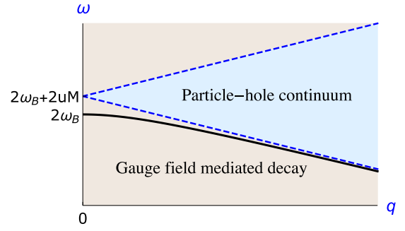
FIG. 1. Magnetic excitation spectrum of an interacting U(1) spin liquid with a spinon Fermi surface. The wedge-shaped (blue) region, bounded by dashed lines, denotes a spinon particle-hole continuum inside which \text{Im } \chi_{\pm}^0(\mathbf{q}, \omega) \neq 0 . The collective spinon spin wave, which is promoted by a short-ranged repulsive interaction u , is shown by the bold black line. The linewidth of this transverse spin wave is determined by the gauge fluctuations, which produce finite \text{Im } \chi_{\pm}^1(\mathbf{q}, \omega) \neq 0 outside the noninteracting spinon continuum [see (11)].
