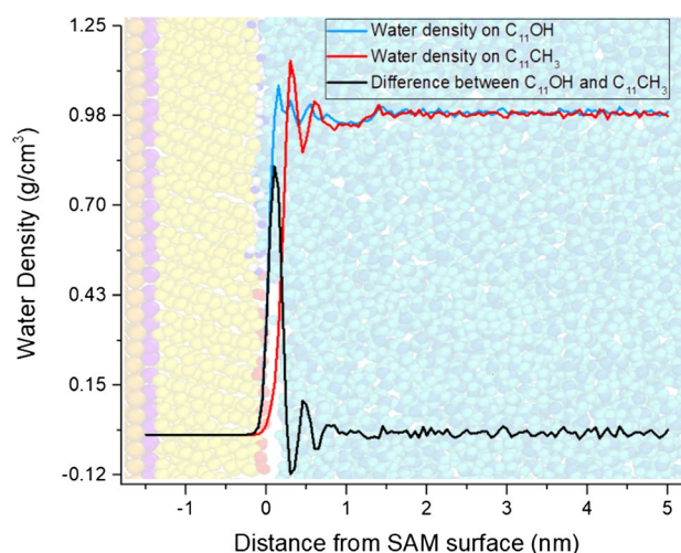
Fig. 5 Water density distribution on C_{11}OH and C_{11}CH_3 SAMs, and the difference in density between the C_{11}OH and C_{11}CH_3 . A faded side-view snapshot of the model system is shown in the background to facilitate correlation between the calculated density and atom positions. The water depletion layer is thicker on the CH_3 terminated SAMs than the OH -terminated SAMs
