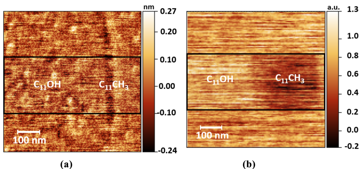
Fig. 2 a Topography and b friction measured using contact mode AFM of C_{11}CH_3 SAMs nanografted into C_{11}OH SAMs. The regions identified by black rectangles were used to calculate the average line profiles reported in Fig. 3a
