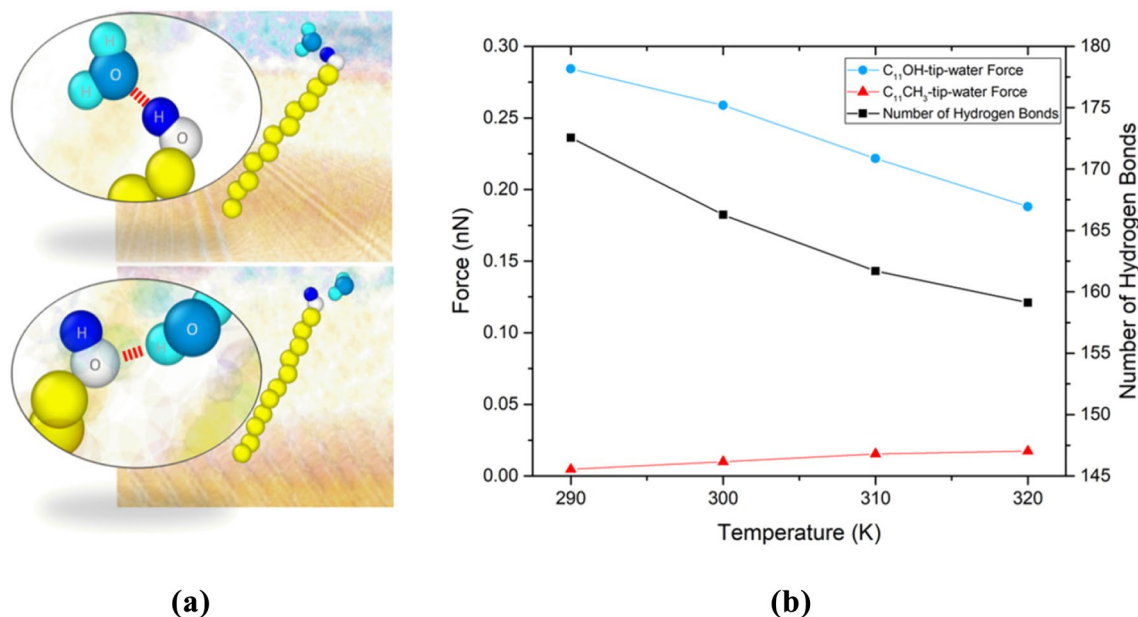
Fig. 6 a Snapshots from the simulation of two H-bonds that are present on the hydrophilic surface, where all atoms except those of interest are faded out for clarity. b Tip-water force and number of H-bonds
