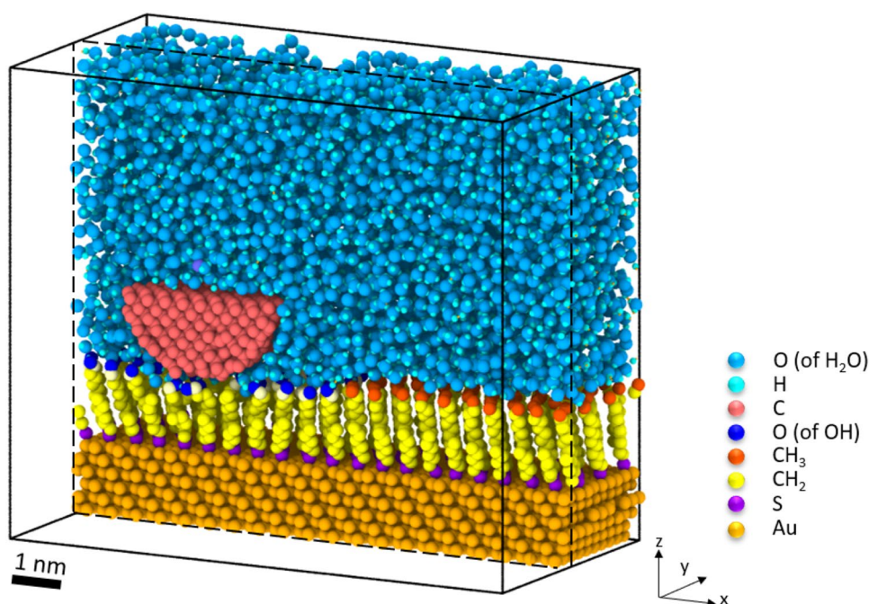
Fig. 1 Perspective view of half of the model showing the tip apex in water sliding on hydrophobic and hydrophilic SAMs on a gold surface. The tip slides in the positive x -direction
