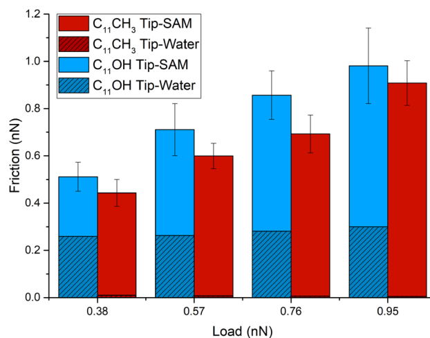
Fig. 4 Average friction force from simulations for the C_{11}OH and C_{11}CH_3 SAMs as a function of normal load. Averages are calculated over the blue and red shaded regions in Fig. 3b and error bars correspond to the standard deviation. The contributions of the tip-water and tip-SAM interactions to the total friction force are shown as patterned vs. solid regions, respectively
