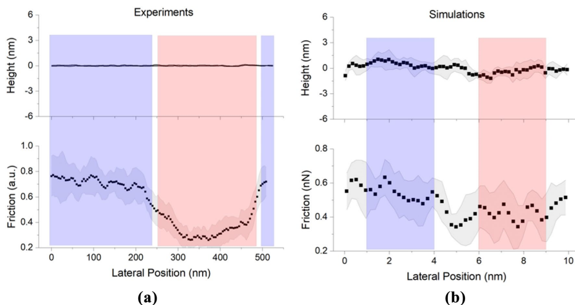
Fig. 3 Average height and friction profiles from a experiments and b simulations illustrating the contrast between C_{11}OH (blue background) and C_{11}CH_3 (red background) SAMs. Symbols represent averages over 15 line traces in experiments and 8 in simulations, and
