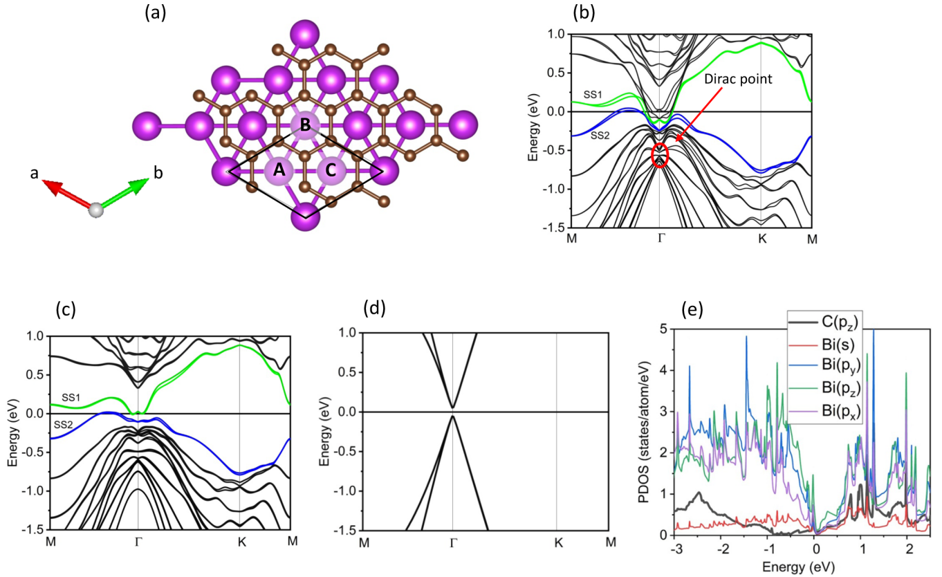
FIG. 1. (a) A top view of the moiré supercell ( \sqrt{3} \times \sqrt{3} ) R30^\circ Gr on (1 \times 1) Bi (111). Brown (the top layer) and pink (the lower layers) colors represent C and Bi atoms, respectively. The solid black lines enclose an in-plane unit cell of the composite. The carbon hexagons have a C_3 symmetry and centered on the Bi atoms marked as A, B, and C, from S, (S-1), and (S-2) surface layers, respectively. (b) Band structure along the high-symmetry lines, using E_F as the reference energy. (c) Band structure for a model system of a Bi thin film, created by removing graphene from the heterostructure. (d) Band structure for another model system of free-standing graphene, created by removing the Bi layers from the composite structure. (e) The projected density of states (PDOS) corresponding to the composite structure, showing negligible hybridization between the carbon-derived and Bi-derived states within 0.5 eV around E_F .
