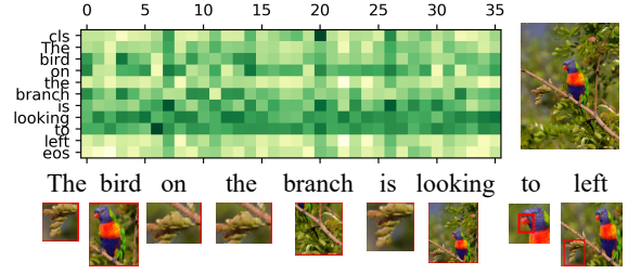
Figure 3: The entity affinity matrix between textual (rows) and visual (columns) modalities. The darker color indicates the higher relevance score. The ROIs with maximum relevance score for each word are shown paired with the words.
