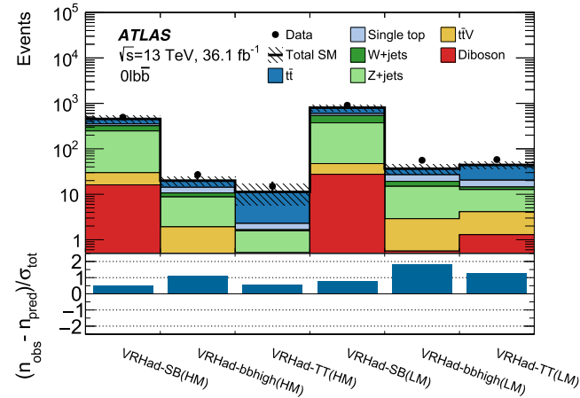
FIG. 3. Comparison of the predicted backgrounds with the observed numbers of events in the VRs associated with the 0\ell b\bar{b} channel. The normalization of the backgrounds is obtained from the fit to the CRs. The upper panel shows the observed number of events and the predicted background yield. All uncertainties are included in the uncertainty band. The lower panel shows the pulls in each VR.
